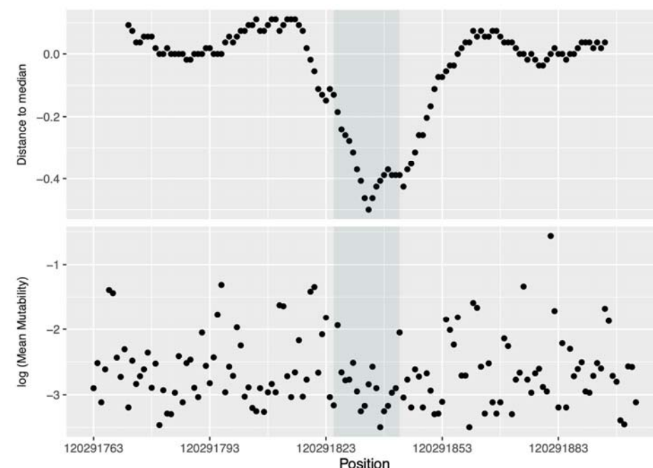
Supplementary Figure 3: (top) Distance to the median proportion of all possible SNVs that are observed in the UK Biobank in 18 bp sliding windows across the length of RNU4-2 . A clear region of depletion compared to the rest of the gene is observed in the centre. (bottom) Log transformation of the mean Roulette 45 mutability across the 3 possible SNVs within a site.
