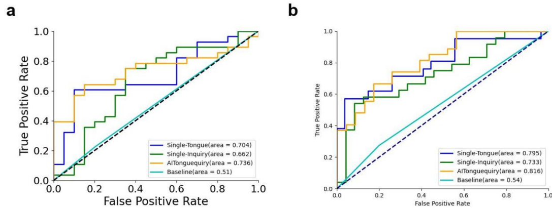
Figure 2. Comparison of ROC curves between different methods for classifying the presence or absence of PLGC and high-risk PLGC in the validation cohorts. (a) Presence or absence of NPLGC/PLGC in the validation cohorts. (b) Presence or absence of low-risk PLGC/high-risk PLGC in validation cohorts.
