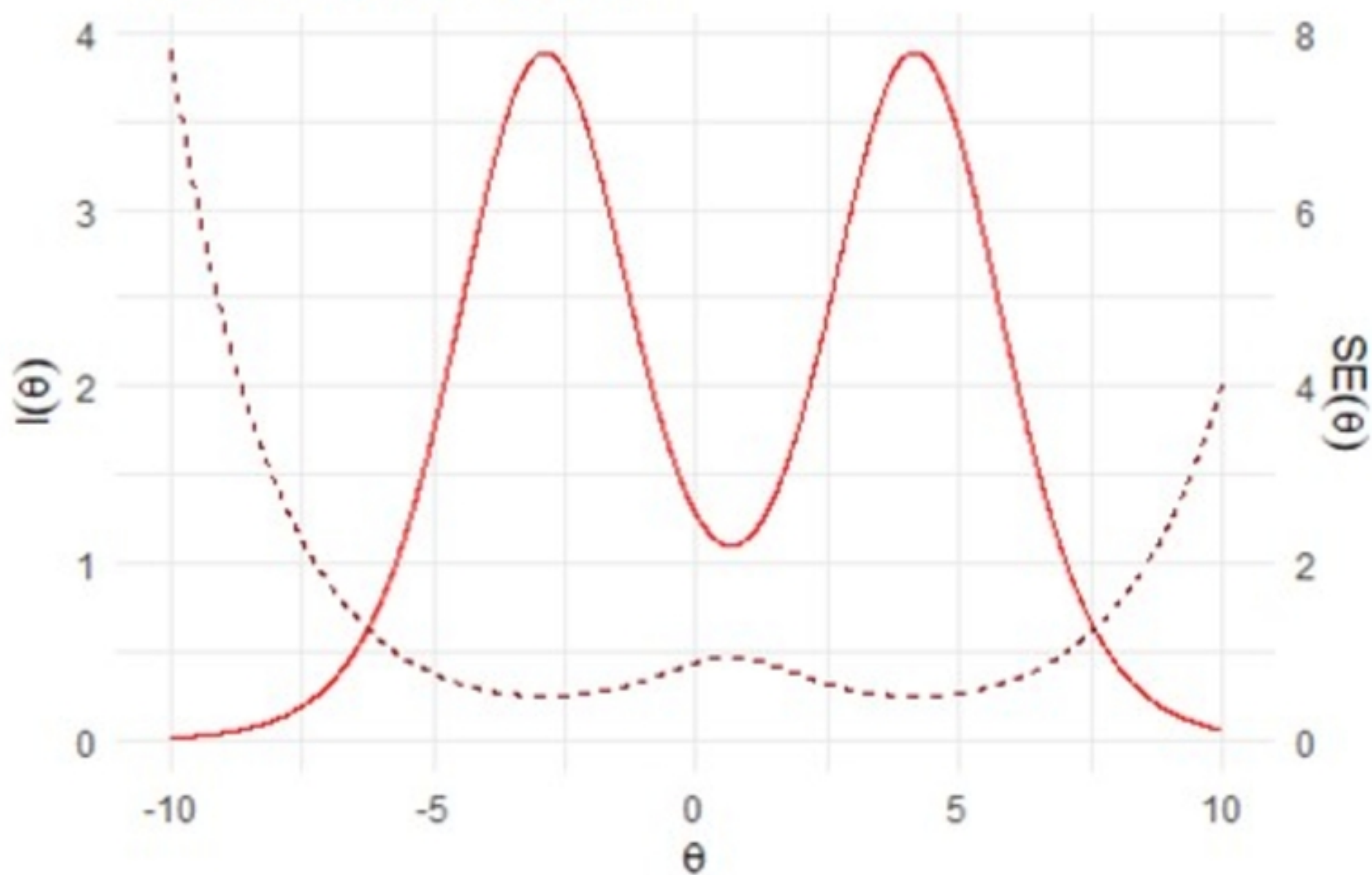
Test Information Curve
