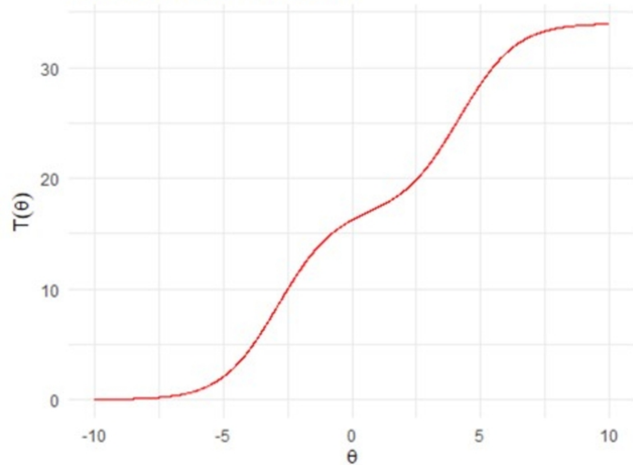
Scale Characteristic Curve
