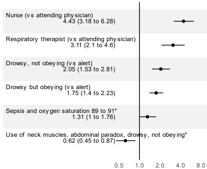
Figure 3: Posterior odds ratios for requesting additional information
