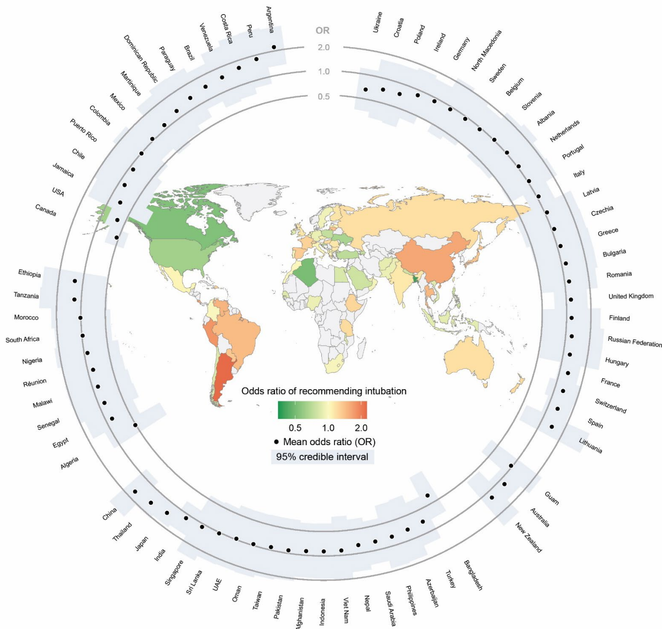
Figure 2: International variation in odds of recommending intubation
