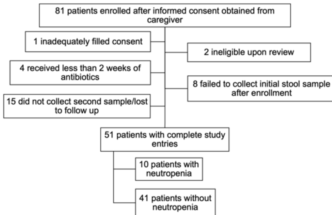
Figure 1. Enrollment Flowchart
