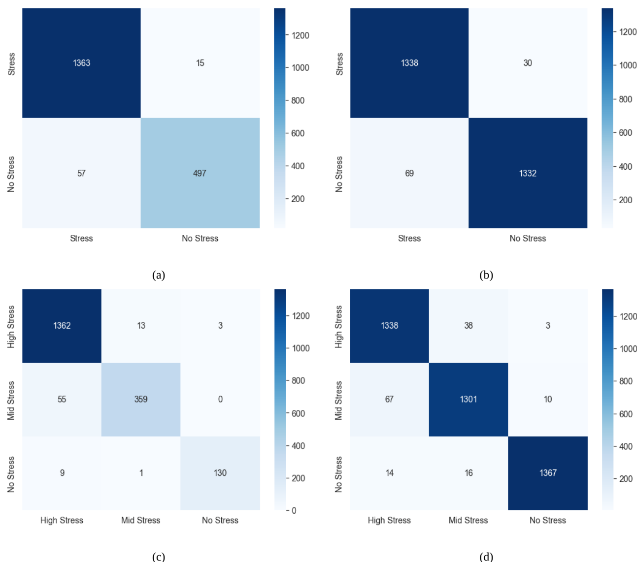
Figure 8 confusion matrix of four scenarios of the SVC model (a) the confusion matrix of two unbalanced classes, (b) the confusion matrix of two classes after using SMOTE, (c) the confusion matrix of unbalanced three classes, (d) the confusion matrix of three classes after using SMOTE.
