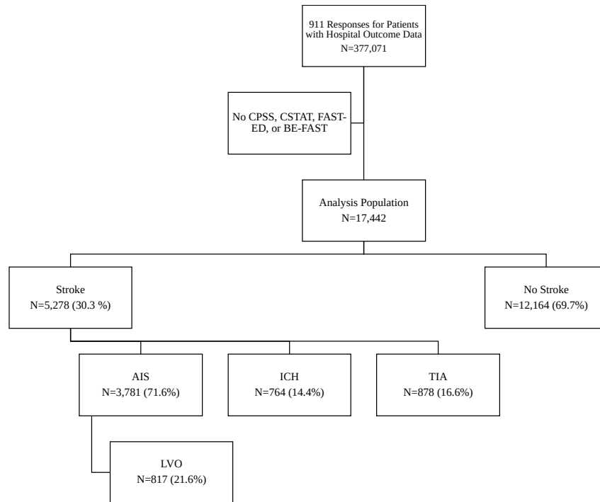
Figure 1: Inclusion of patients for analysis and hospital/emergency department stroke diagnoses. CPSS: Cincinnati Prehospital Stroke Scale; C-STAT: Cincinnati Stroke Triage Assessment Tool; FAST-ED: Field Assessment Stroke Triage for Emergency Destination; BE-FAST: Balance Eyes Face Arm Speech Time; AIS: Acute Ischemic Stroke; ICH: Intracerebral Hemorrhage; TIA: Transient Ischemic Attack
