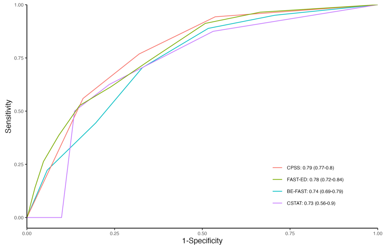
Figure 2: ROC curves for prehospital stroke severity scales. CPSS: Cincinnati Prehospital Stroke Scale; C-STAT: Cincinnati Stroke Triage Assessment Tool; FAST-ED: Field Assessment Stroke Triage for Emergency Destination; BE-FAST: Balance Eyes Face Arm Speech Time
