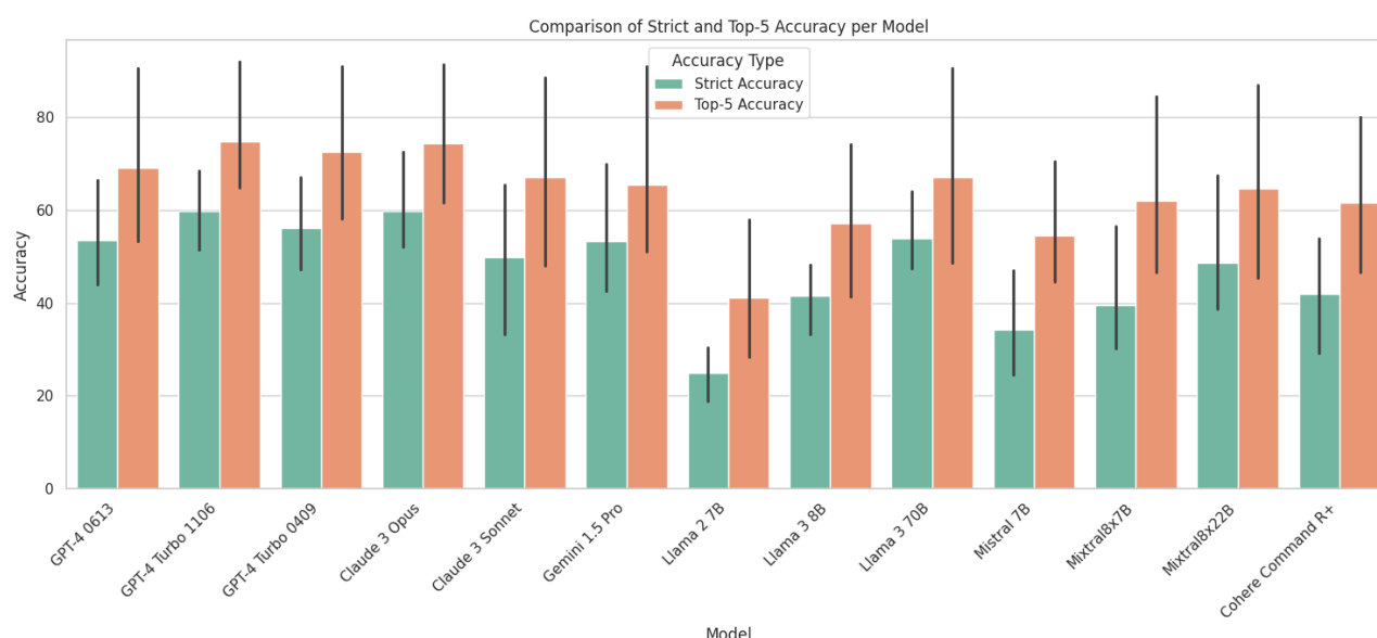
Figure 1: Comparative diagnostic accuracy of all the models on all datasets.
