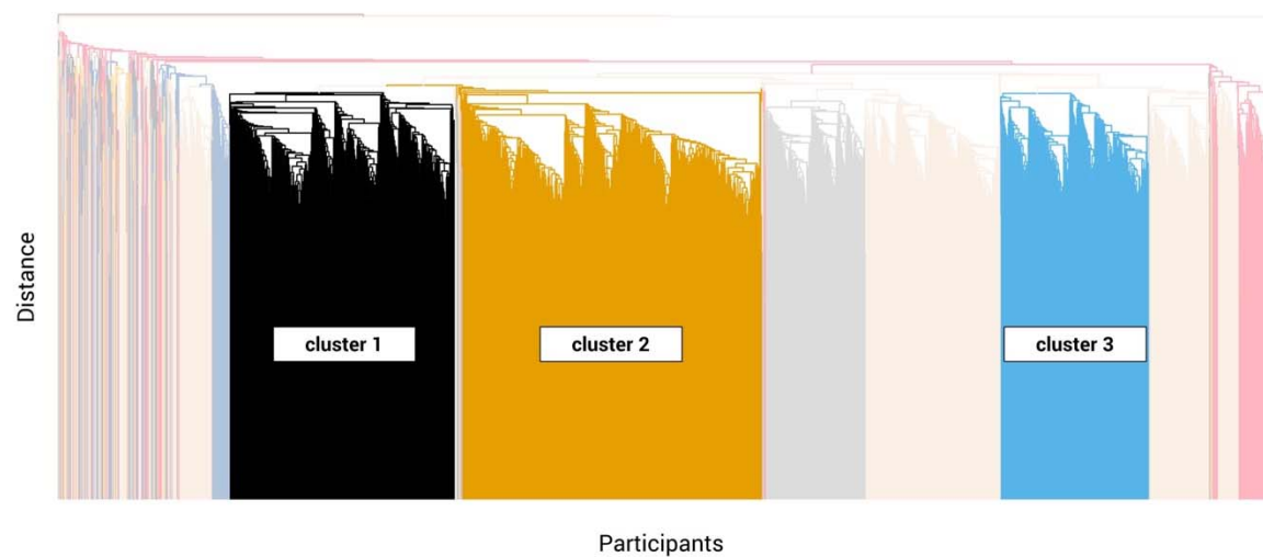
Figure 2. Dendrogram for the hierarchical agglomerative clustering
