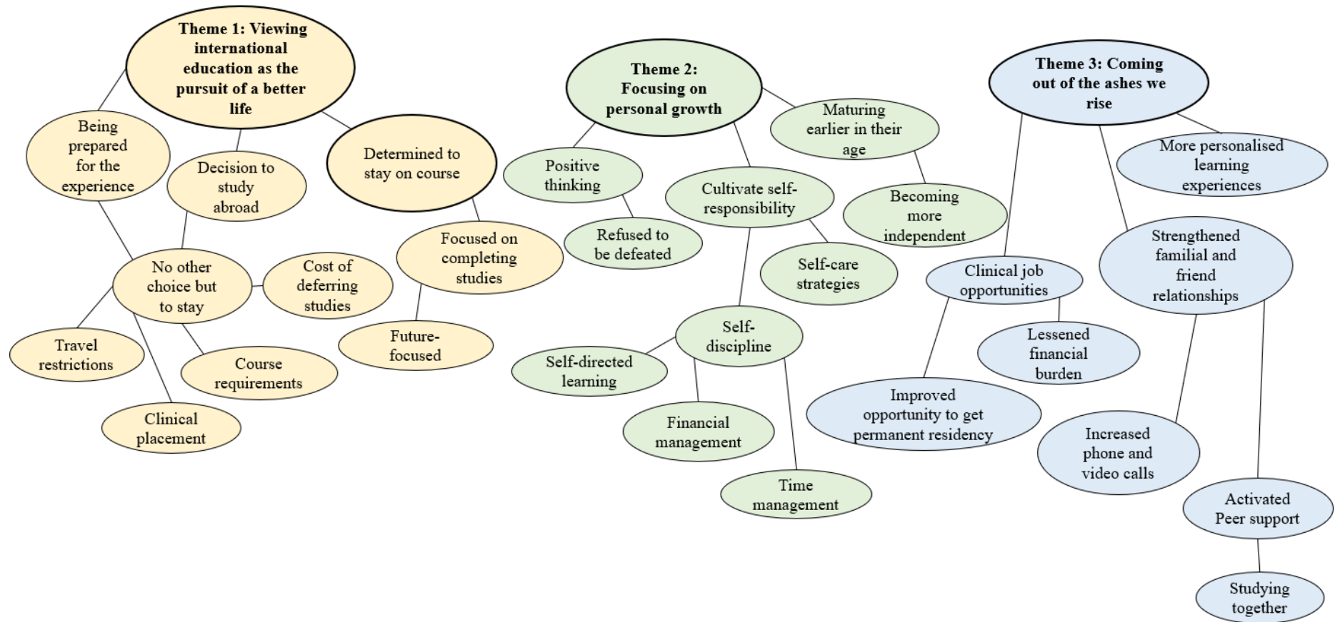
Figure 1. Coding tree
