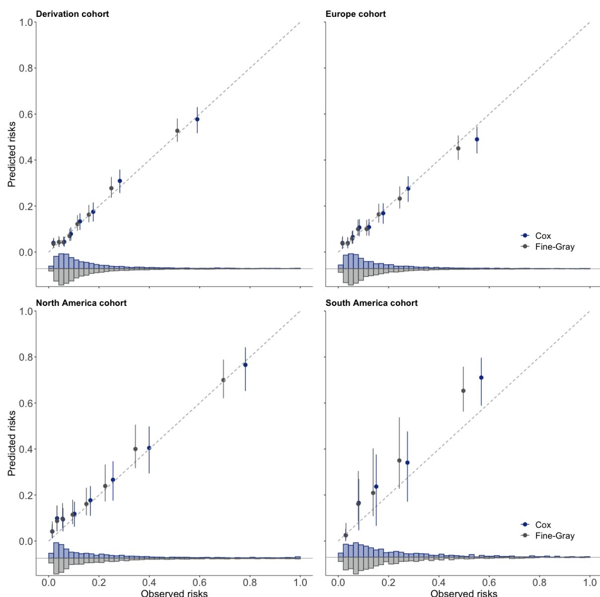
Figure 4. Calibration curves assessed at 7 years post risk-evaluation in the derivation and external validation cohorts. Calibration plots are presented at 7 years post risk-evaluation in the derivation cohort and in the European and North American external validation cohorts, and at 5 years post-risk evaluation in the South American external validation cohort. In each group (8 groups for the derivation, European and North American cohorts, and 5 groups for the South American cohort), the median of the predicted risks (one minus the individual predicted survival probabilities for the Cox model and the individual predicted risks, i.e., cumulative incidence, for the Fine-Gray model) was plotted against the observed event probability estimated by (one minus) the Kaplan-Meier estimator for the Cox model and the Aalen-Johansen estimator for the Fine-Gray model, respectively. The diagonal line at the origin represents the perfectly calibrated model. The histograms represent the distribution of the Cox and Fine-Gray models' individual predicted risks.
