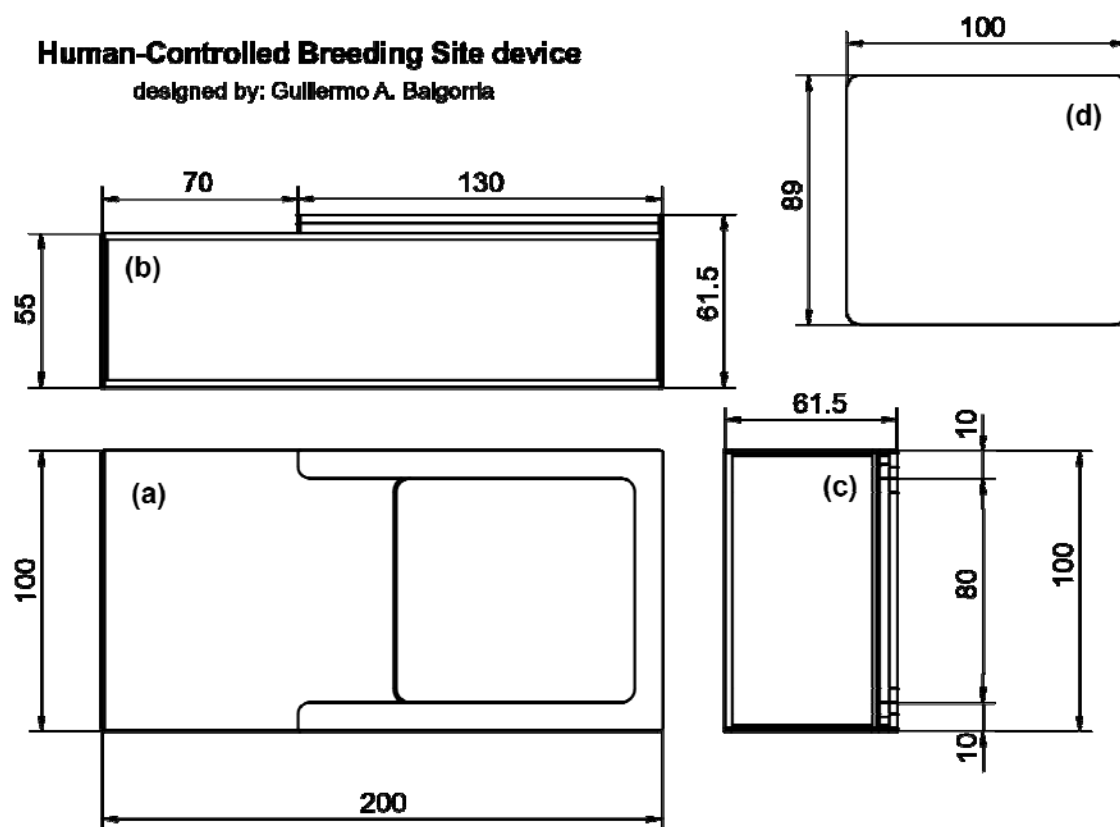
Figure 1: Design drawings of the HCBS device, showing (a) top view of the body, (b) side view of the body, (c) front view of the body, and (d) top view of the slicing cap. Measurements are in millimeters (mm).
