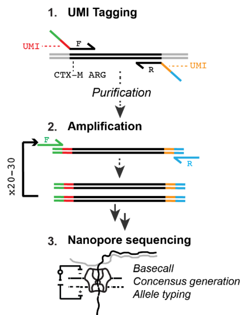
113 Figure 1: Schematic of UMI PCR Protocol. UMIs are added to each template molecular. Tagged molecules 114 are subsequently amplified and sequenced. Consensus sequences are generated from binning by UMIs.
