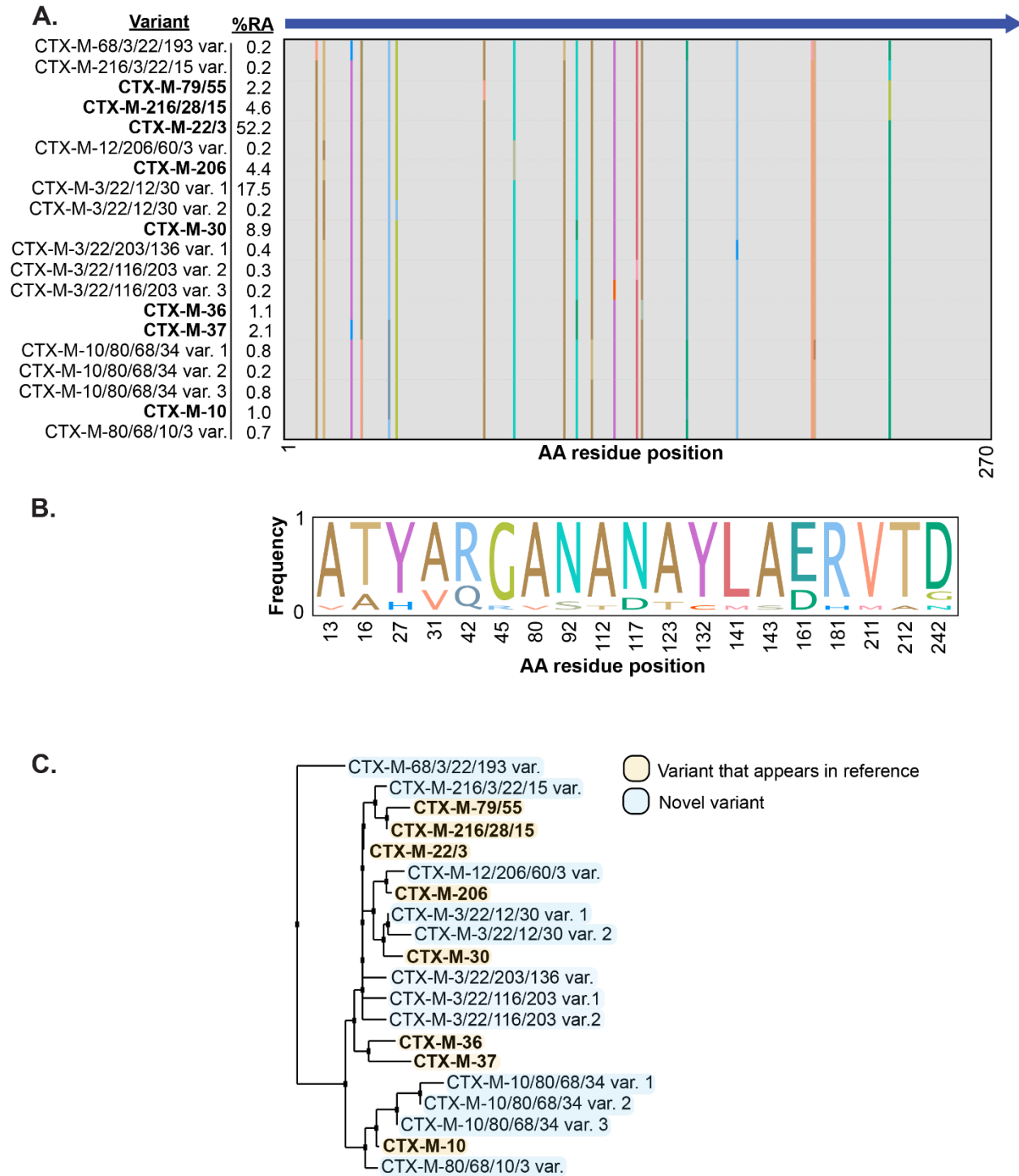
Figure 3: A.) Location of observed mutations across the top 20 protein variants (amino acid level) of the CTX-M gene. B.) Frequency of amino acid substitutions at loci with multiple residues based on unique variants and not abundance weighted C.) Phylogenetic tree of the top 20 protein variants using nearest neighbor joining.
