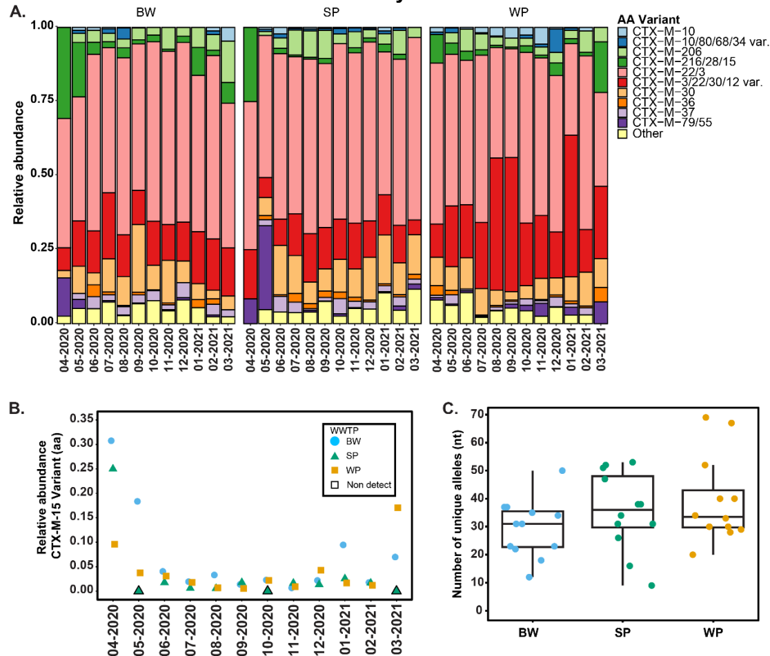
Figure 2: A.) Relative abundance of the top 10 most common protein variants across all samples. B.) Relative abundance of the CTX-M-15 containing protein variant (CTX-M-216/28/15), which has high clinical relevance, across all samples. C.) Number of unique nucleotide alleles by WWTP.
