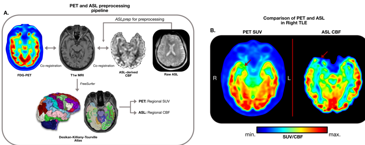
Figure 1 – Image processing pipeline: Panel A. demonstrates the imaging pipeline used to pre-process the PET and ASL data for each subject. ASL data was preprocessed with ASLprep which performed cerebral blood flow (CBF) estimation and T1w MRI co-registration of the resulting CBF map. FDG-PET images were co-registered to the T1w image of each subject as well. Using FreeSurfer, Desikan-Killiany-Tourville atlas parcellations were extracted from each subject's T1w image, and the corresponding PET SUV and ASL CBF values within each of these parcels was estimated. Panel B. shows the PET SUV and ASL CBF (Gaussian smoothed with \sigma=3 ) maps for the same subject. Red arrow points to a region of congruent hypometabolism and hypoperfusion.
