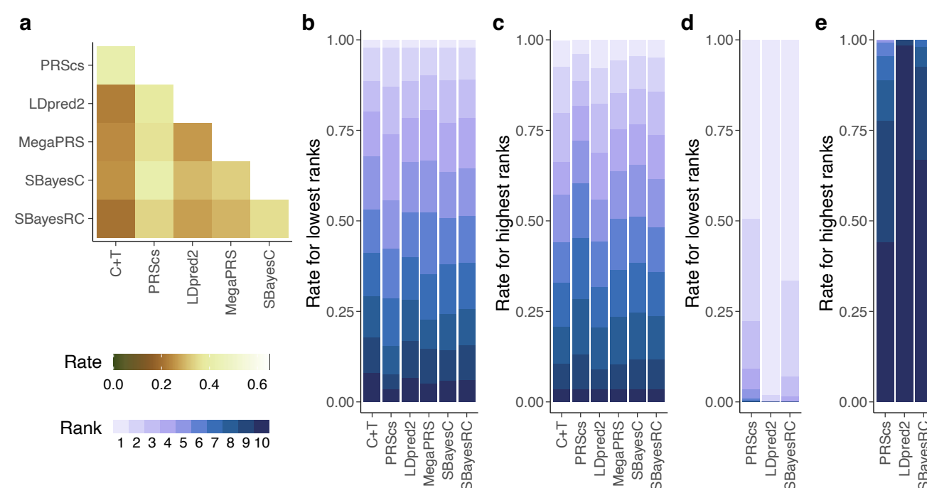
Figure 1. Prominent inconsistency of embryo selection rank across PRS methods.
