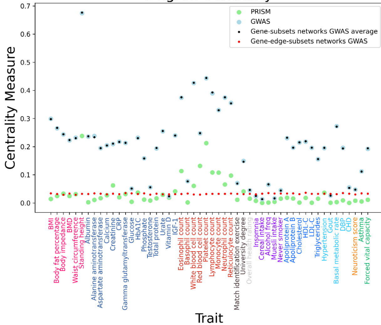
Degree Centrality
