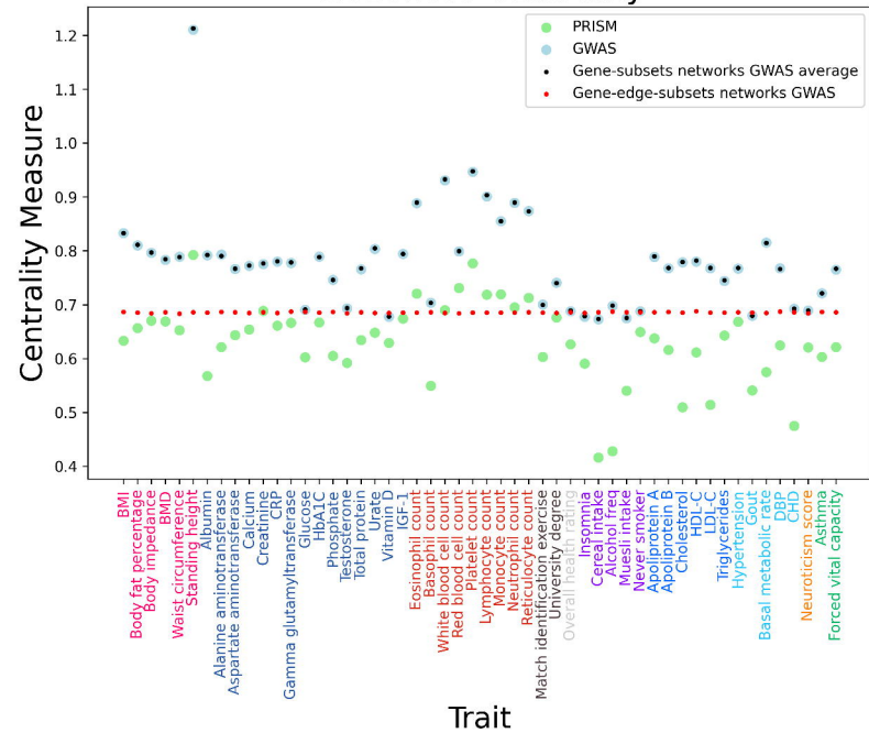
Closeness Centrality
