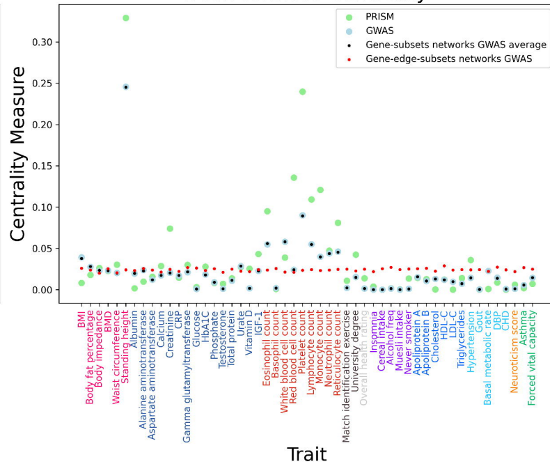
Betweenness Centrality
