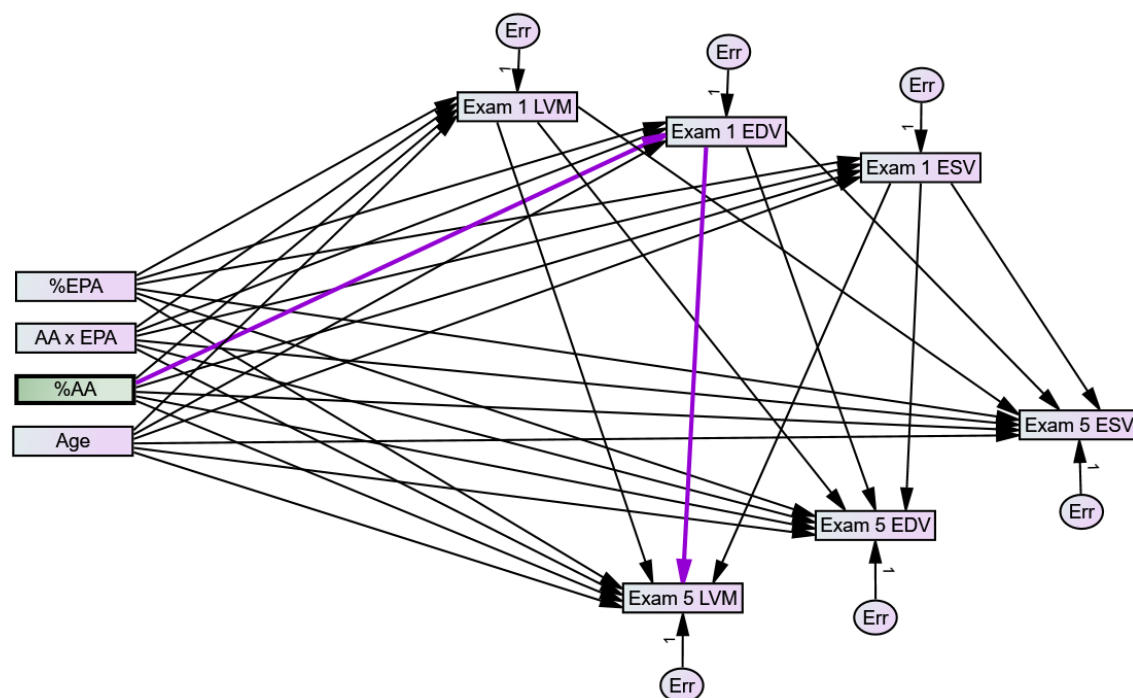
Figure 3: Final pathway model: The final model is depicted using standard format where observed exogenous and endogenous variables are represented by rectangles and unobserved exogenous variables using circles. Paths are represented as linear, single headed arrows and covariances are represented using curved, double-headed arrows. The model allows for indirect effects of AA, EPA, and AA×EPA on Exam 5 (direct arrows to Exam 5 outcomes) or indirect paths by way of Exam 1 outcomes (2 step combination of path to Exam 1 outcome followed by path from Exam 1 to Exam 5 outcome). Highlighted in dark violet is an example of a conditional, indirect effect of AA and EPA on Exam 5 LVM by way of their effect on Exam 1 EDV. Details can be found in Supplemental Tables .
