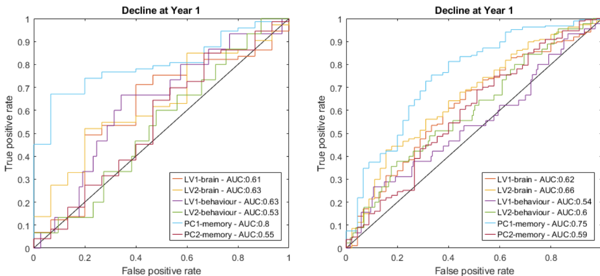
Figure 5. ROC analysis
