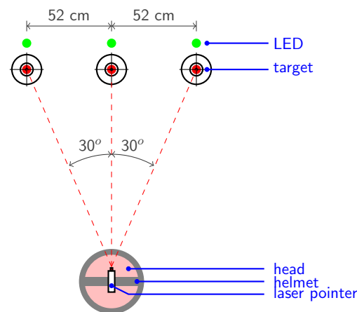
FIG. 1: Schematic representation of the real-world DidRen laser test; view from above.
