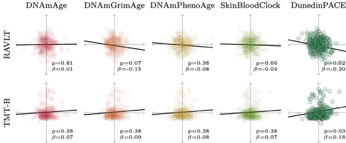
Fig. 2 Scatterplots showing individual data and model fit lines from linear regressions from the stage 2 training dataset of age- and sex-adjusted candidate methylation ages (MA) and memory (Rey Auditory Verbal Learning Test, immediate recall (RAVLT), upper row) and executive function (Trail Making Test, part B (TMT-B), lower row). \beta represents the linear regression coefficient of each MA and the corresponding False Discovery Rate-corrected p -value
