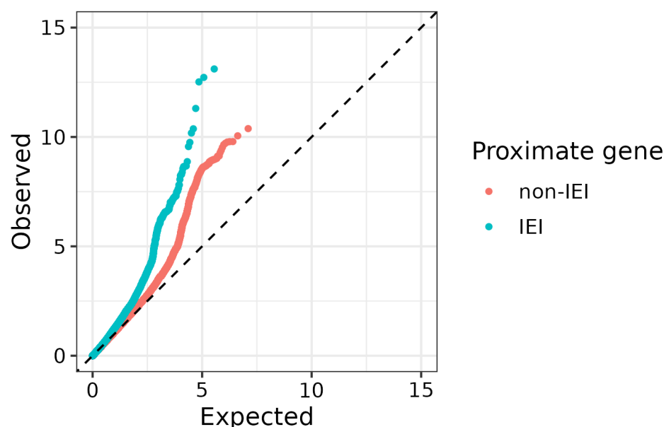
Figure 2. A quantile-quantile plot depicting the empirical quantiles of the SIgAD meta-analysis p-values on a -\log_{10} scale, coloured according to their proximity to IEI or non-IEI genes. Each point corresponds to a SNP, with the y-coordinate giving the SNP's observed -\log_{10} p-value in the meta-analysis and the x-coordinate giving the -\log_{10} p-value expected if there were no associated SNPs. The dotted line y = x depicts the trajectory of the data where the observed distribution matches the expected uniform distribution, i.e. the scenario where all SNPs are null for association with SIgAD.
