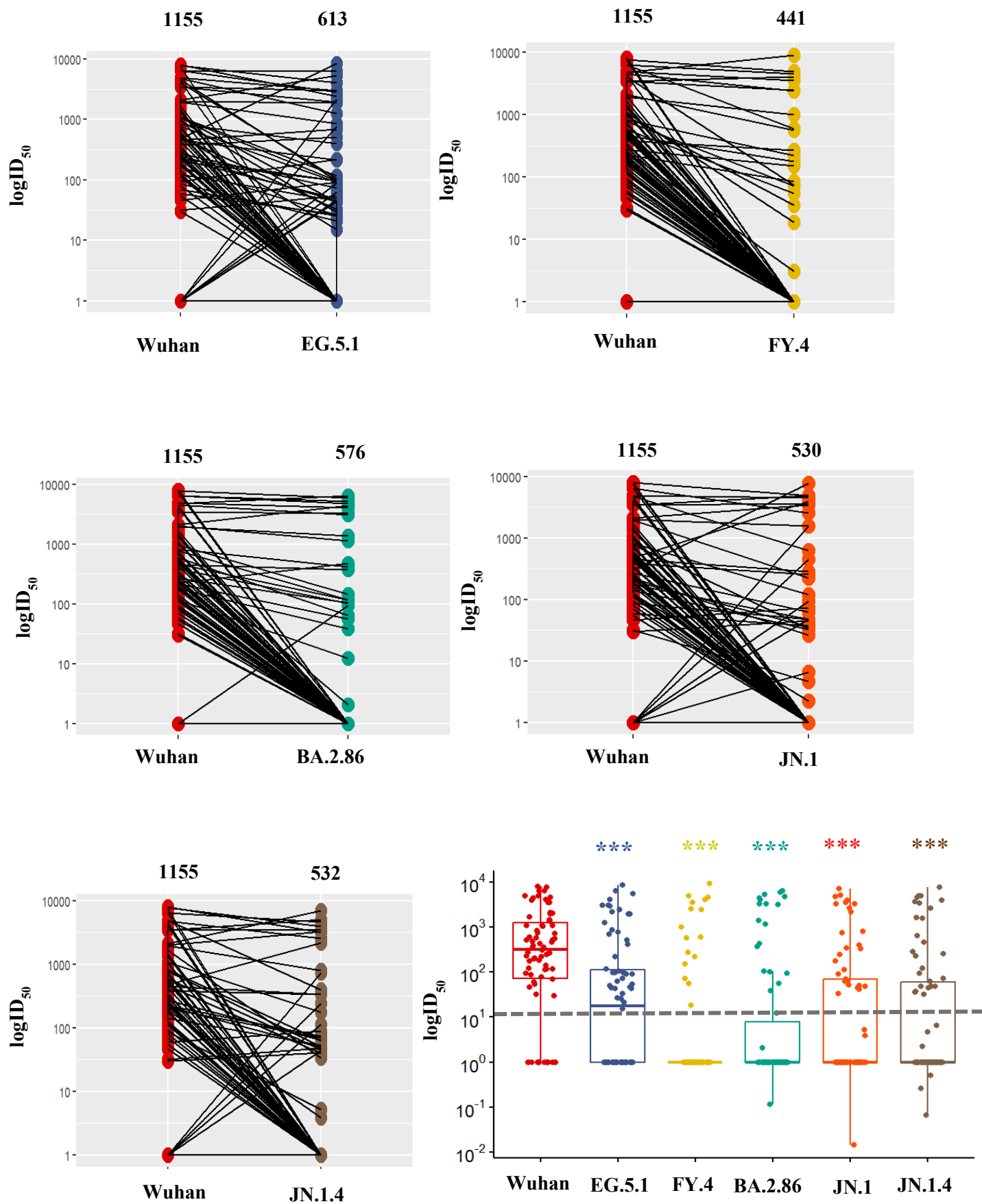
124 Figure 2: A comparison of inhibitory dilutions ( ID_{50} ) between wildtype and omicron variants
