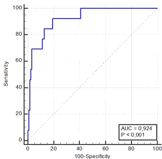
Figure 4. AUC for probability of having a positive genetic test.
