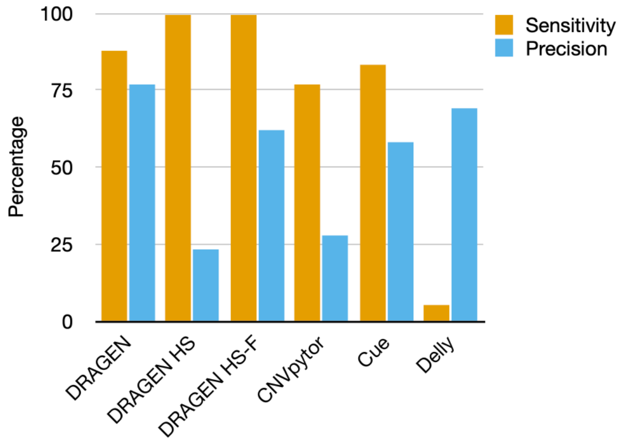
Figure 4. Virtual Gene-Panel Performance.
