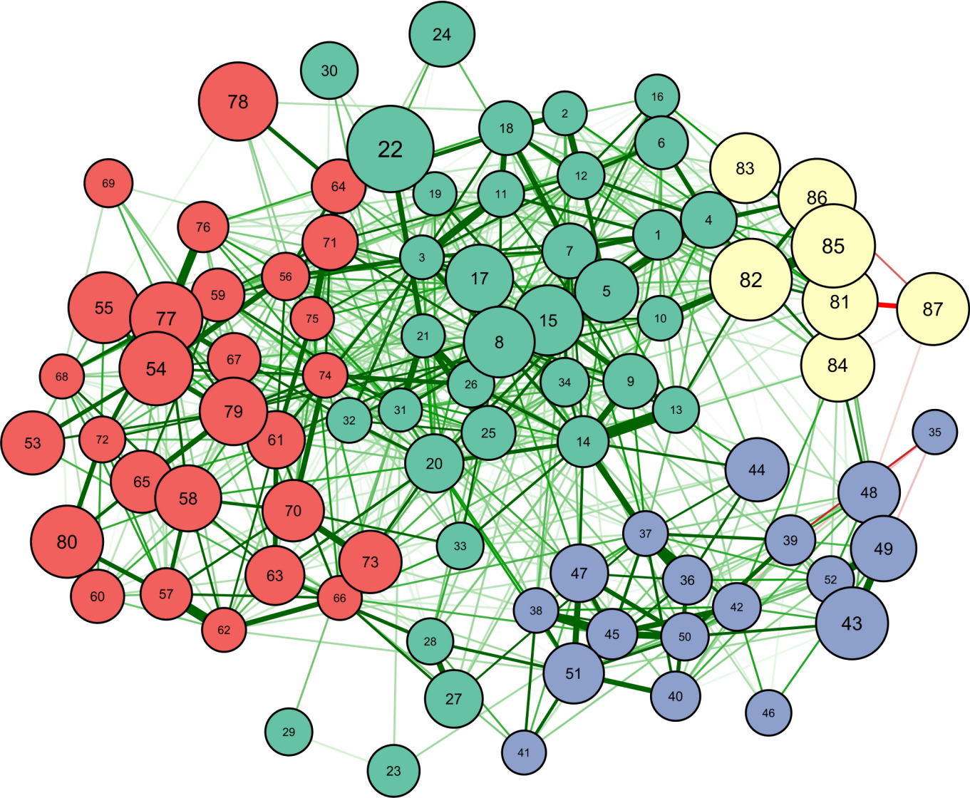
EGA model of the O-LIFE – new 4 factors
