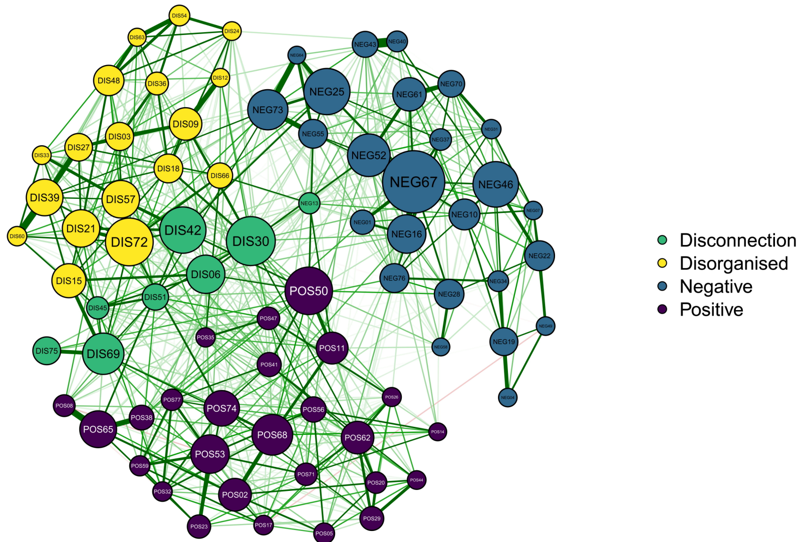
EGA model of the MSS – 4 FACTORS + Betweenness centrality
