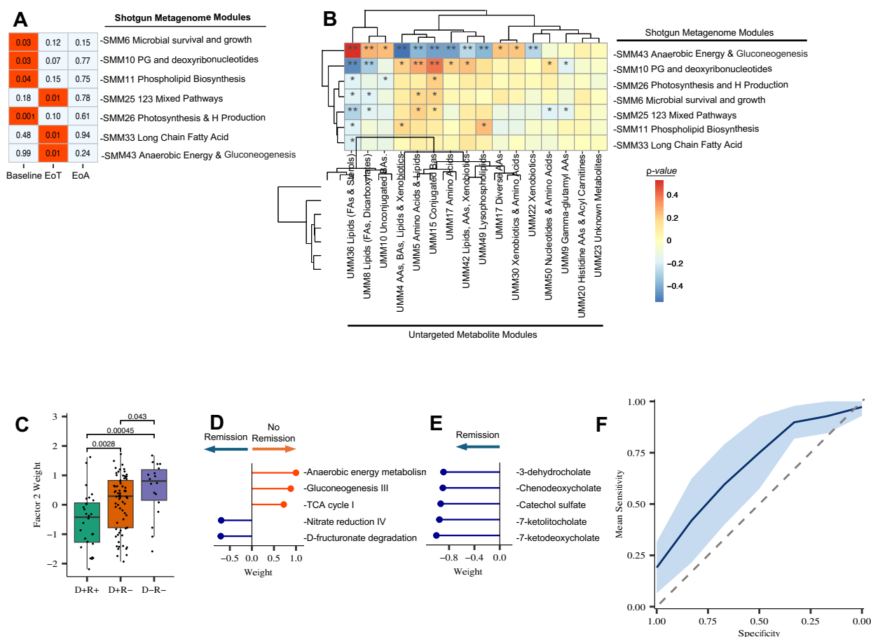
Figure 3. a , Association between shotgun metagenomic module (SMM) eigengenes and POIT outcomes (ANOVA, adjusted for age). b , Heatmap showing Spearman correlation results between POIT-associated Untargeted Metabolomics Modules (UMMs) and Shotgun Metagenomics Modules (SMMs). Asterisk “*” represents P < 0.05 , and double Asterisk “**” represents P < 0.01 . c , Factor 2 from MOFA analyses is the most significantly differential Factor between POIT response groups and weighted significantly higher in no remission groups compared to D+R+ group ( P < 0.05 , Wilcoxon signed-rank test). d , Top 5 microbial pathways contributing the Factor 2 weight contains Gluconeogenesis and anaerobic energy metabolism pathways. e , Top 5 metabolites contributing the Factor 2 weight contains bile acid metabolites. f , The model’s predictive ability expressed as the AUC computed from 100 times repeated five-fold cross-validation. Blue line shows the average across the 100 times repeated five-fold cross-validations with the shaded area representing the 95% CI (mean AUC \pm standard deviation). The dashed diagonal line represents random chance. Error bars represent standard deviation.
