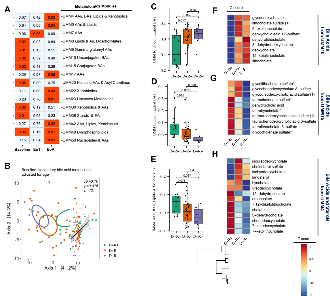
Figure 2. a , Association between untargeted metabolomics module (UMM) eigengenes and POIT outcomes (ANOVA, adjusted for age). b , Ordination of baseline secondary bile acid metabolites ( n=43 , R^2=0.10 ; P<0.015 , adjusted for age), PERMANOVA analyses based on Euclidian dissimilarity metrics. c , Difference in baseline Module Eigengenes (ME), which were determined based on WGCNA analyses (see Method Section) and represents a measure of the joint abundance profile of a specific module, of UMM10, d , UMM15 Unconjugated BAs module, and e , UMM4 between POIT-outcome groups (Wilcoxon signed-rank test). f , Z-scores of each bile acid-related metabolites of UMM10, g , UMM15 and, h , UMM4 in each POIT-outcome groups (D+R+, D+R-, and D-R-). Blue colors represent low z-scores thus low abundance and red colors represent high z-score and higher abundance. Error bars represent standard deviation.
