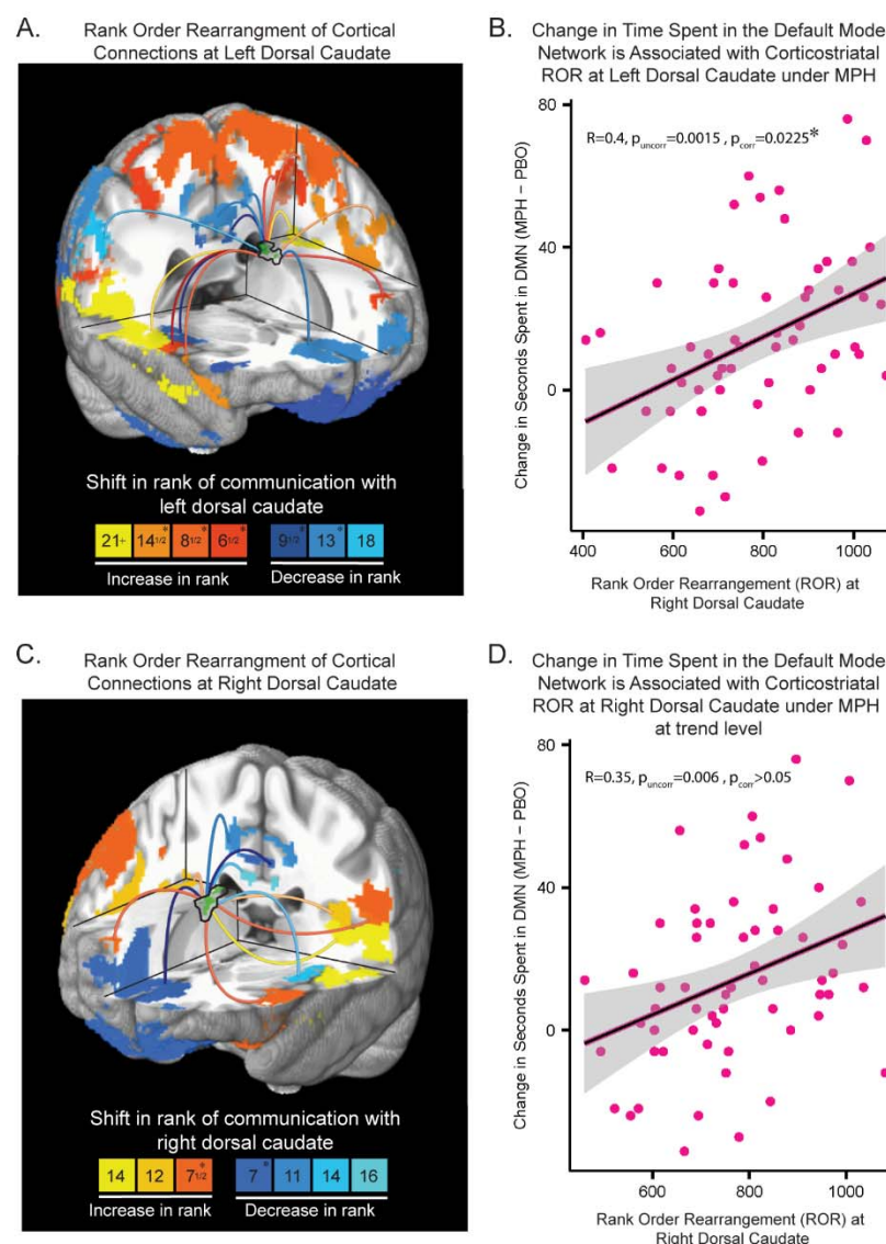
Figure 5. A and C. ROR at left dorsal caudate (A) and right dorsal caudate (C), depicting absolute change in relative connectivity between multiple cortical regions and the dorsal caudate node under MPH compared to PBO: Green regions are the data-driven striatal nodes of significant MPH-induced ROR previously identified by a voxel-wise paired t-test. Cortical regions are color coded to depict how their relative connectivity strength with the specified caudate node, or 'rank of communication', shifts under MPH compared to under PBO. Regions shown shift at least 5 ranks. Color key at bottom indicates magnitude of change in rank where * indicates a mean magnitude of change for that color – this value only varies by \pm 2 values at maximum. Exact amount of change per significant cortical region is depicted in supplementary material figure S3. B and D. Correlations between ROR at left dorsal caudate (B) and at right dorsal caudate (D) and change in time spent (seconds) in the DMN under MPH compared to PBO. MPH: methylphenidate; PBO: placebo; DMN: default mode network; *p_{\text{corr}} < 0.05 .
