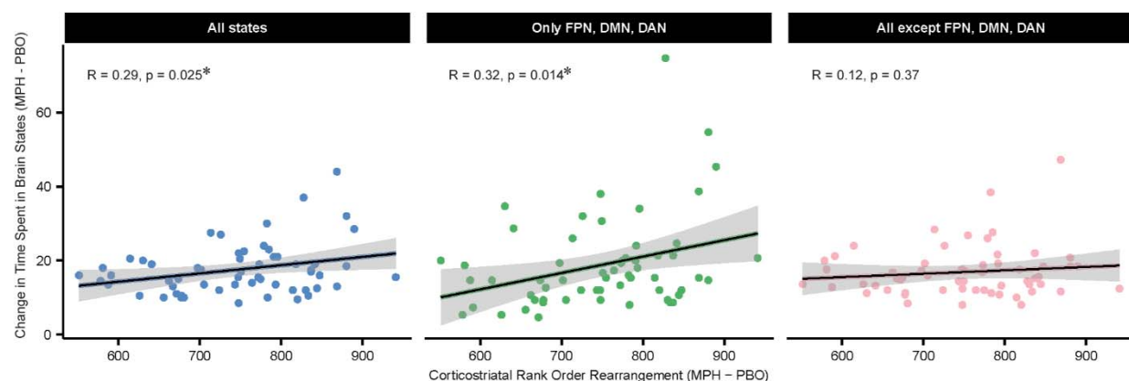
Figure 4. Change in network temporal dynamics is associated with altered corticostriatal rank order rearrangement under MPH. Change in network temporal dynamics is operationalized as the sum, for each state tested, of the absolute value of the difference in total time spent in the state (MPH-PBO). Three panels vary by y-axis where left panel y = change in time spent in all states, middle panel y = change in time spent in only FPN, DMN and DAN states, right panel y = change in time spent in all states except FPN, DMN, and DAN states. All Y-axis measures were divided by the number of states summed. MPH: methylphenidate, PBO: placebo; DMN: default mode network; DAN: dorsal attention network; FPN: frontoparietal network.
