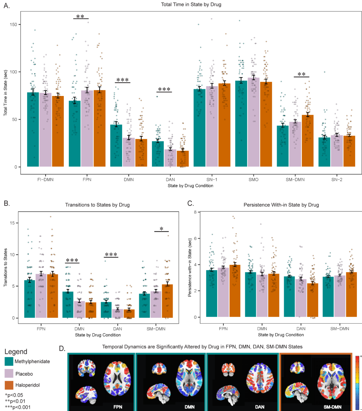
Figure 1. A. MPH increased time spent in DMN and DAN states and decreased time spent in FPN state. HAL increased time spent in SM-DMN state. B. MPH increased transitions to DMN and DAN states while HAL increased transitions to SM-DMN state. C. Neither MPH nor HAL altered time spent persisting within DMN, DAN, FPN states or SM-DMN state. D. A visualization of FPN, DMN, DAN and SM-DMN states of which dynamics are significantly altered by MPH (outlined in green) or HAL (outlined in orange). -1 is most negative relative activation; +1 is most positive relative activation. MPH: methylphenidate; HAL: haloperidol; FI-DMN: fronto-insular default mode network state; FPN: frontoparietal control network state; DMN: default mode network state; DAN: dorsal attention network state; SN-1: salience network state 1;
