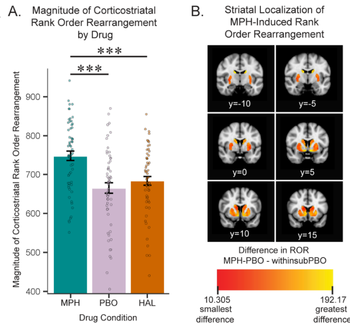
Figure 3. Methylphenidate Significantly Heightens the Magnitude of Rank Order Rearrangement in Corticostriatal Connectivity Profile
