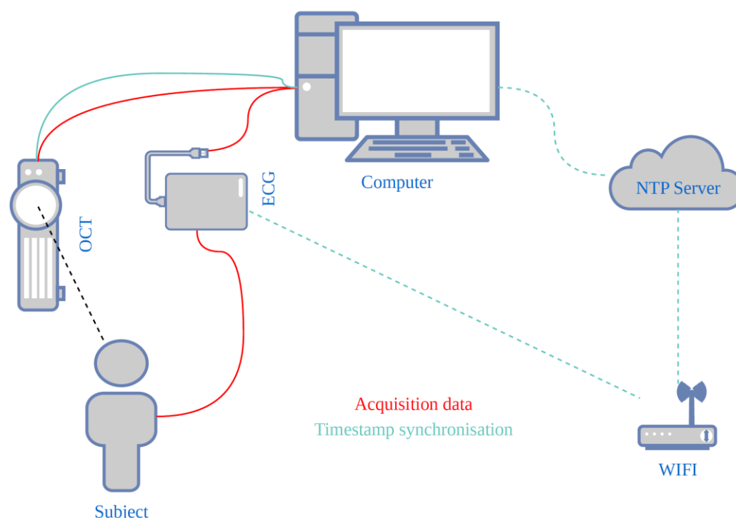
Fig. 1. Electrocardiogram-coupled optical coherence tomography.
