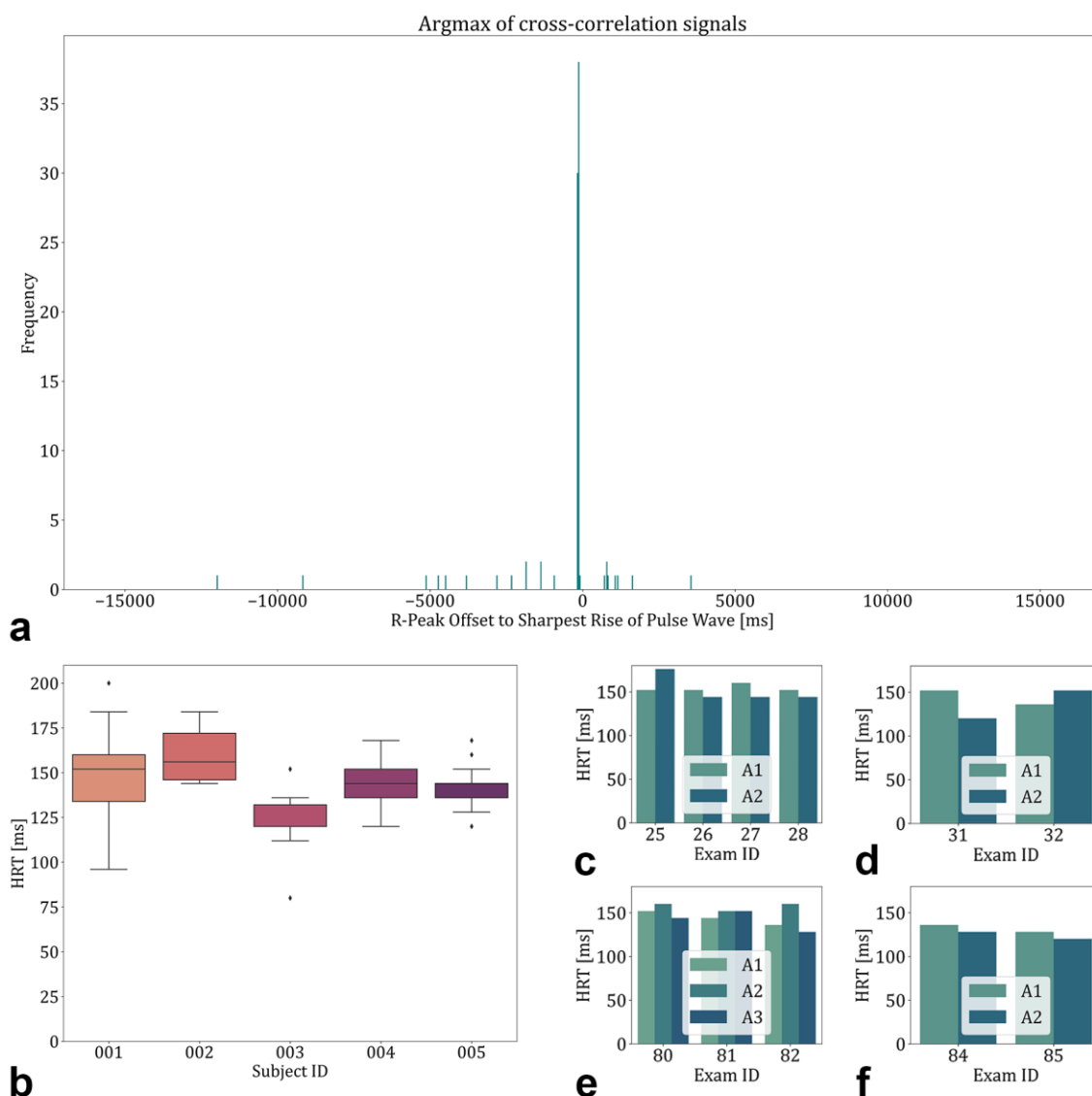
Fig. 5. Heart-retina time (HRT) results overview. a Histogram plot with a bin width of 50ms for the argmax of the cross-correlation signals showing that the most probable delay between the R-Peak and the arrival of the pulse is within one cardiac cycle. b HRTs of the five included subjects showing good intrasubject and inter-subject reproducibility. c-f HRTs of different acquisitions within the same vessels.
