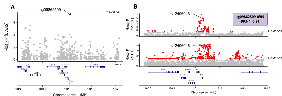
Figure 4 Regional plots for the sentinel CpG gene pair showing the highest posterior probability of colocalization. Two types of regional association plots are shown for cg09862509- IER5 : A. Associations of CpGs surrounding cg09862509 with DCM from discovery-stage EWAS (MAGNet). The displayed region is centered on cg09862509 (red; bordered) B. Genetic associations for cg09862509 and IER5 . Genetic associations were obtained for a +/-500kb region centered on the instrumental variable used in SMR assess causal relationships between cg09862509 methylation and IER5 gene expression (meQTL from MAGNet; eQTL from GTEx.) Posterior probability of colocalization between cg09862509 meQTLs and IER5 eQTLs was 0.91. Gene tracks for all regional plots consist of protein-coding genes obtained from Ensembl Release 75 (last release based on hg19 assembly).
