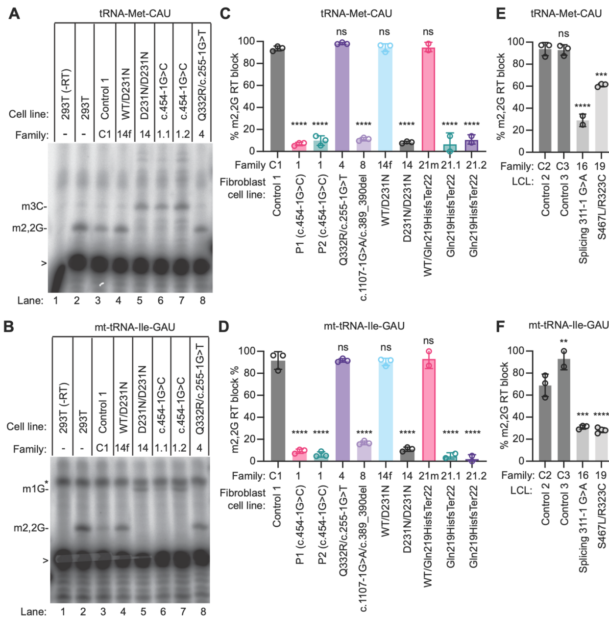
Figure 5. Patient cells with biallelic TRMT1 variants exhibit a reduction in m2,2G modifications in tRNAs. (A, B) Representative gels of primer extension assays to monitor the presence of m2,2G in tRNA-Met-CAU and mt-tRNA-Ile-GAU from the indicated cell lines. m3C 20 , 3-methylcytosine; m2,2G 26 , dimethylguanosine; m1G 9 , 1-methylguanosine; >, labeled oligonucleotide used for primer extension; *, background signal. (C through F) Quantification of m2,2G formation by primer extension for the indicated tRNAs. N=3. Error bars represent standard deviation from the mean. Statistical analysis was performed using one-way ANOVA. For (C) and (D), the means of each column was compared to the Control 1 cell line. For (E) and (F), the means of each column was compared to the Control 2 cell line. *P ≤ 0.05; **P ≤ 0.01; ***P ≤ 0.001; ****P < 0.0001; ns, non-significant, P > 0.05.
