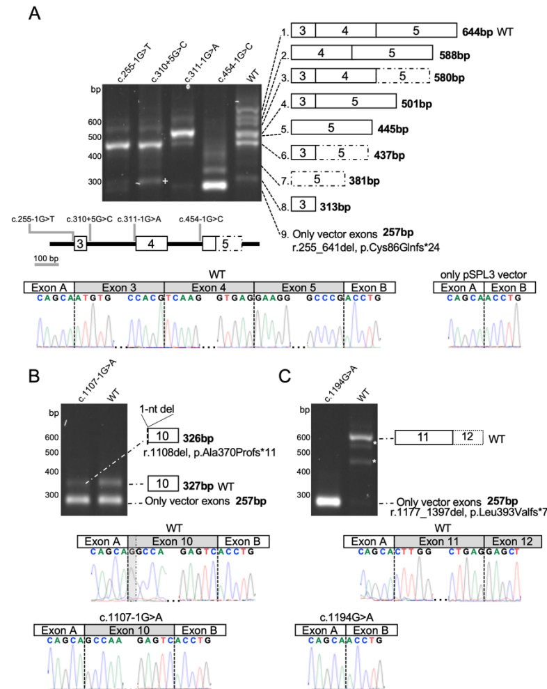
Figure 3. TRMT1 variants induce splicing defects. Wild-type (WT) and mutant minigenes were transfected in HEK293T cells and their RNA subjected to RT-PCR. (A) RT-PCR for WT and mutant minigenes showed complex splicing patterns. We obtained sequencing validation for all except amplicon 2. The presence of additional bands in the WT is attributed to alternative splicing and was quantified in Supplementary Table 5. The only protein coding transcript expressed in the brain includes exons 3-5 that has been eliminated or reduced due to the four variants. The upper left panel shows the RT-PCR agarose gel with the splicing schematic shown for each band to the right. The variant schematic is shown below. Sanger sequencing results of the RT-PCR showing the correctly spliced WT with the deleterious variant effect, exon skipping, as shown by the presence of only pSPL3 vector. The dotted box represents the short version of exon 5. (B) RT-PCR of the c.1107-1G>A results in loss of the native splice acceptor site and cryptic splice activation leading to loss of a G and a frameshift. The left panel shows the RT-PCR agarose gel with the splicing schematic shown for each band to the right. Exon 10 with 1 bp deletion is represented with a dotted line corresponding to the position of the single bp deletion. (C) RT-PCR of the c.1194G>A variant leads to a frameshift due to exon skipping of exons 11 and 12 leading to a frameshift. Asterisks represent assay artifacts. The left panel shows the RT-PCR gel with the splicing schematic shown to the right. Assay design captured part of exon 12 that was correctly spliced in the WT control.
