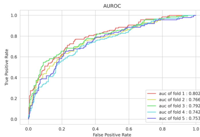
Supplementary Figure S6. AUPRC (A) and AUROC (B) for malnutrition prediction model - BioClinicalBERT
