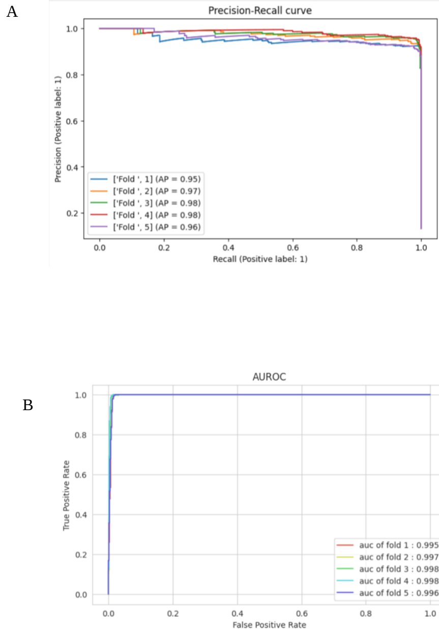
Supplementary Figure S3. AUPRC (A) and AUROC (B) of malnutrition note identification model - BioClinicalBERT
