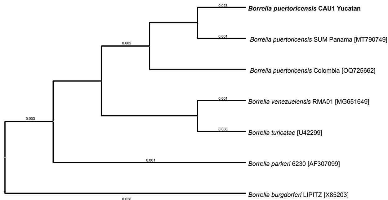
Fig 3. Maximum-likelihood tree constructed from flaB partial sequences of various Borrelia species. The analysis was performed with the amino acid substitution model Blosum62. Sequences generated in this study are in bold. Numbers represent bootstrap support generated from 1000 replications. The NCBI accession numbers are in brackets and Borrelia burgdorferi was used as outgroup.
