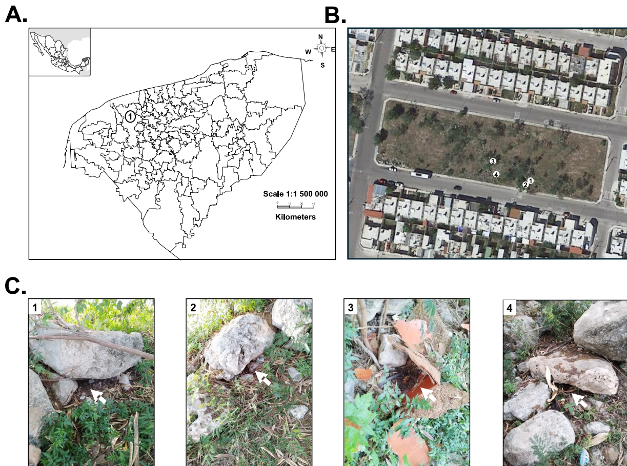
94 95 Fig 1. Collection and identification of Alectorobius ( Ornithodoros ) puertoricensis in 96 Yucatan, Mexico. Shown is a map of the state of Yucatan, the number 1 in the map shows 97 the location of Merida city, left upper corner map shows the location of Yucatan in Mexico 98 (A). Collection site was in Ciudad Cauce, here in a terrain map and the numbers indicate 99 location of the burrows (B). The white arrows in (C), panels 1 through 4, point to where 100 ticks were collected. In (C), C1 to C4 point to the respective locations in panel (B). Terrain 101 maps were obtained from Google maps and used under the “principles of fair use” 102 ( https://about.google/brand-resource-center/products-and-services/geo-guidelines/ ).
