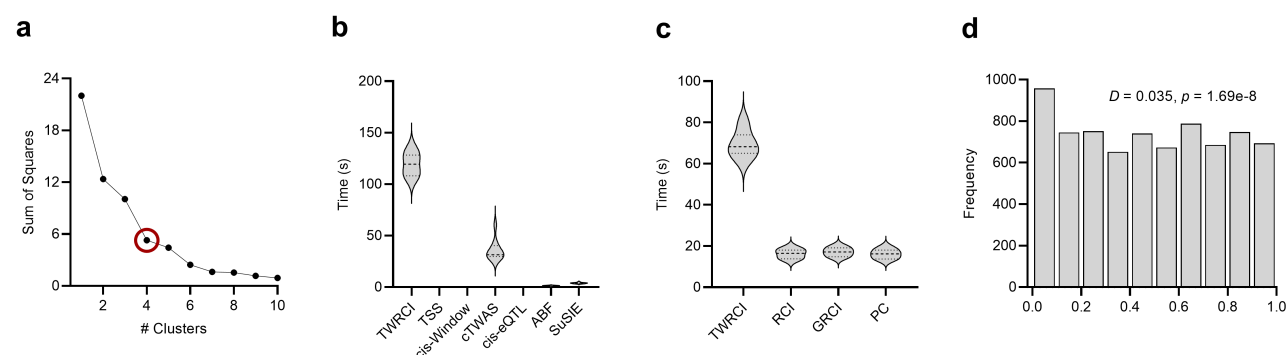
Supplementary Figure 2. Additional results for COPD. (a) Sum of squares plot for hierarchical clustering using Ward's method revealed four clusters according to the elbow method, or the cluster size with the maximum distance from the imaginary line drawn between the first and last cluster sizes. TWRCI took the longest time to complete in annotation (b) and the second longest time to complete in graph reconstruction (c); SIGNET required 8690 seconds on average in reconstruction, so we do not plot its timing results. RCI, GRCI and PC took the shortest amount of time to reconstruct the causal graph because they ignore the genetic variants. (d) Histogram of Pearson correlation test p-values computed between variants annotated to the phenotype and gene expression levels. The p-values did not follow a uniform distribution according to the Kolomogorov-Smirnov test with statistic D indicating the presence of confounding between the variants annotated to the phenotype and gene expression.
