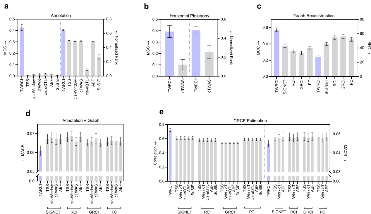
Figure 3. Synthetic data results in terms of (a) direct causal annotation, (b) annotation focused on horizontal pleiotropy only, (c) graph reconstruction, (d) combined annotation and graph reconstruction, and (e) CRCE estimation accuracy. Four of the graphs summarize two evaluation metrics. Arrows near the y-axis denote whether a higher (upward arrow) or a lower (downward arrow) score is better. We do not plot the results of cis-eQTL and SuSIE in (d) due to much worse performance. Error bars correspond to 95% confidence intervals. The cis-window and cTWAS algorithms have the exact same CRCE estimates in (e) because accounting for horizontal pleiotropy in cTWAS does not change the conditioning set \mathbf{D} in Equation (1); we thus denote cis-Window and cTWAS as Win/cT for short. TWRCI in purple outperformed all algorithms across all nine evaluation metrics.
