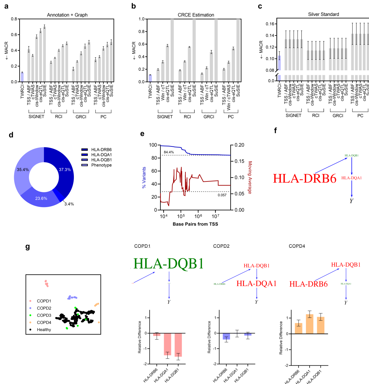
Figure 4. Results for COPD. (a) TWRCI outperformed all other combinations of algorithms in direct causal annotation and graph reconstruction by achieving the lowest MACR; error bars correspond to one standard error of the mean in accordance with the one standard error rule of cross-validation 26 . (b) TWRCI similarly achieved the lowest MACR for CRCE estimation. (c) Silver standard genes exhibited the smallest correlation with the phenotype after partialing out the root causal genes inferred by TWRCI. (d) More than 35% the causal variants exhibited horizontal pleiotropy. TWRCI annotated the remaining causal variants to three gene expression levels. (e) TWRCI assigned approximately 84% of the causal variants to genes located on different chromosomes. Most causal variants annotated to a gene on the same chromosome fell within a one megabase distance from the TSS (blue, left). The average magnitude of the regression coefficients decreased slowly with increasing distance starting from about 100 kilo-bases from the TSS (red, right); the dotted line again corresponds to variants on different chromosomes. (f) The COPD-wide causal graph revealed multiple HLA type II genes as root causal. (g) UMAP dimensionality reduction revealed three clusters of COPD patients well-separated from the healthy controls. The directed graphs highlighted different root causal genes within each of those three clusters. Finally, bar graphs revealed different mean gene expression levels relative to healthy controls in each cluster; error bars denote 95% confidence intervals in this case.
