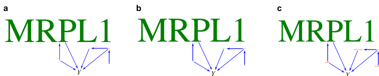
Supplementary Figure 5. Replication results in an independent set of patients from the UK Biobank (dataset ukb-d-I9_IHD). We summarize results for (a) all patients, (b) cluster one and (c) cluster two. TWRCI again identified MRPL1 as a root causal gene with a large positive CRCE.
