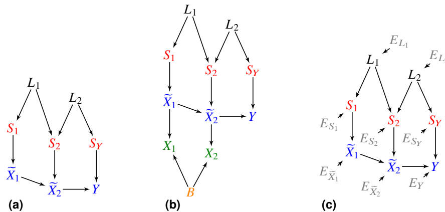
Figure 6. (a) An example of a DAG over Z . In (b), the additional vertices X denote counts corrupted by batch B effects and Poisson measurement error. (c) We can also augment the DAG in (a) with root vertex error terms E .
