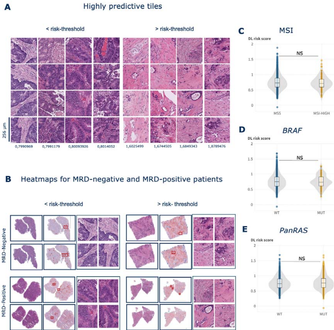
Figure 3: Morphological and molecular features of the DL risk score
