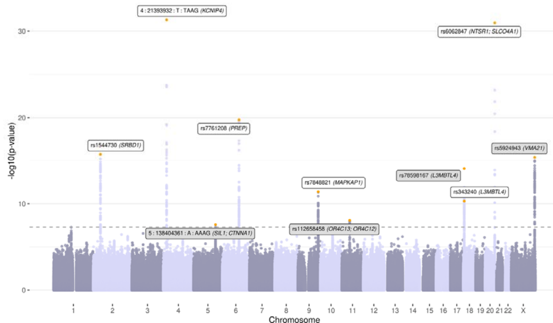
Figure 2. Manhattan plot for the multi-trait GWAS of chronic dry cough and ACEi-induced cough. The dotted grey line represents the genome-wide significance threshold ( p -value < 5 \times 10^{-8} ). Sentinels are highlighted orange and mapped genes are labelled; novel sentinels are highlighted grey.
