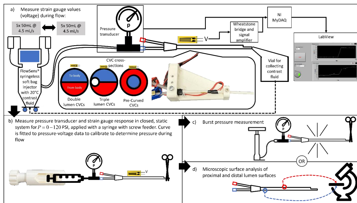
Figure 1: The experimental setup for testing the central venous catheters: a) the catheters with strain gauges are clamped and connected to a contrast medium injector with a pressure transducer placed at the inlet of the catheter. b) The strain gauges are then calibrated through static pressure. The pressure transducer values are stored together with the strain gauge voltages. Next the pressure transducer and strain gauge voltages are processed, and a curve fit is generated. Intraluminal pressure during injection is determined through this curve fit. c) catheters are finally pressurized until burst; or d) microscopic surface analysis is performed on the lumina of 1 sample of each catheter types tested.
