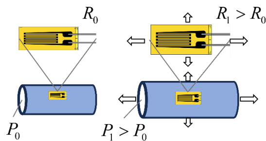
Figure 2: Working principle of a strain gauge. The strain gauge is placed on a surface and the resistance R is continuously measured, of which the value is R_0 at rest with intraluminal pressure P_0 . When the material stretches, e.g. due to a higher intraluminal pressure P_1 , the strain deforms with the material. The resistance of the deformed gauge R_1 will increase due to the increase in length and decrease in cross-sectional diameter of the wire. This can then be measured as a voltage change when amplified in a Wheatstone bridge.
