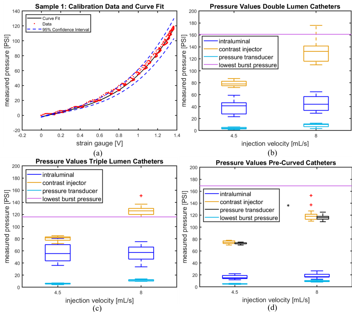
Figure 3: a) The calibration data, fitted 3 rd -order polynomial and its 95% confidence bounds of catheter sample 1, used to determine intraluminal pressure with the strain gauge. b-d) Boxplots of the pump pressures, intraluminal strain gauge pressures and pressure transducer values at injection velocities 4.5 mL/s and 8 mL/s, and the burst pressures of b) the double lumen catheters; c) the triple lumen catheters; and d) the pre-curved catheters. n=4 applies to (b-d) *Only 3 samples have been tested
