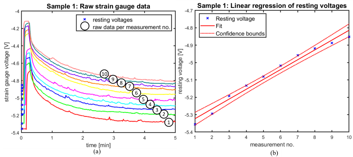
Figure 4: Representative regression plot of catheter 1 showing the trend in resting voltages throughout the measurements. Patterns are similar throughout the tested catheters. a) shows the raw strain gauge data over the 5-minute testing period of measurements 1 through 10 in catheter 1, as indicated by the numbers in the graph; and b) displays the regression analysis of the resting voltages as indicated in a).
