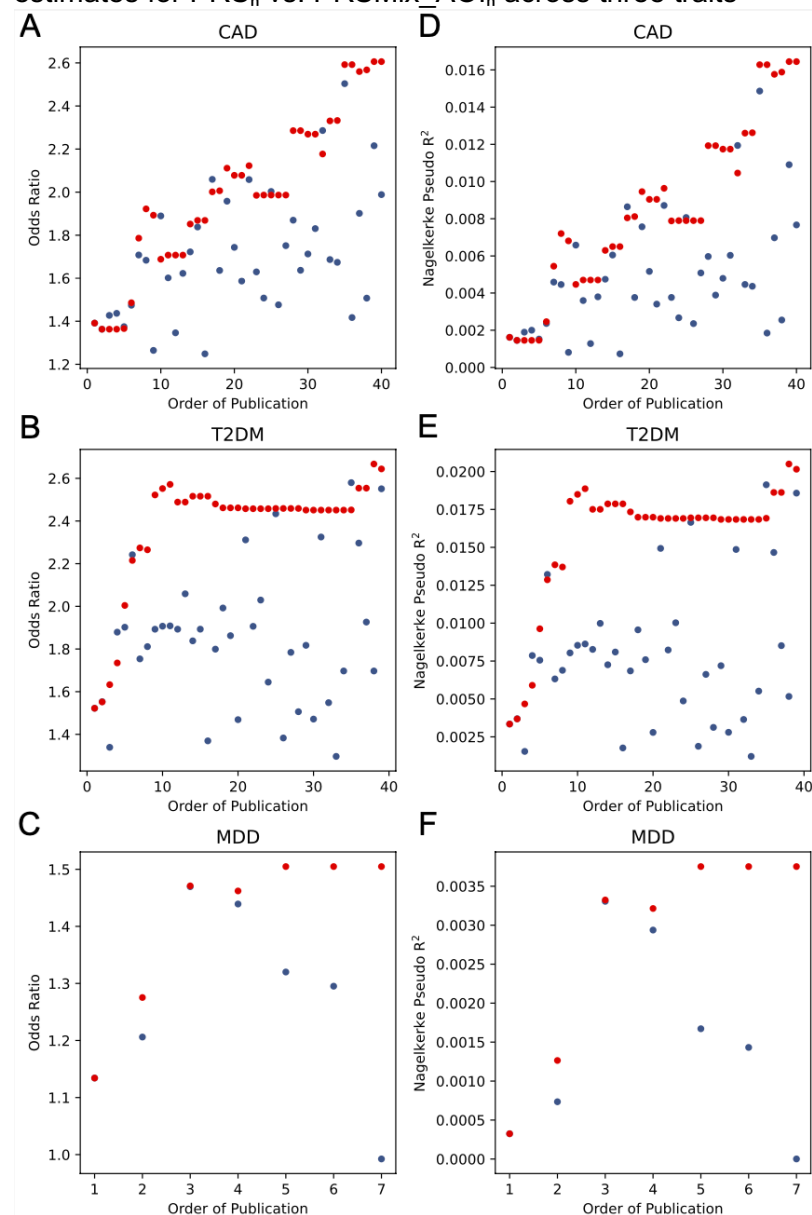
Extended Figure 2: Chronologic trends in association strength and variance explained estimates for PRS n vs. PRSMix_AOI n across three traits
