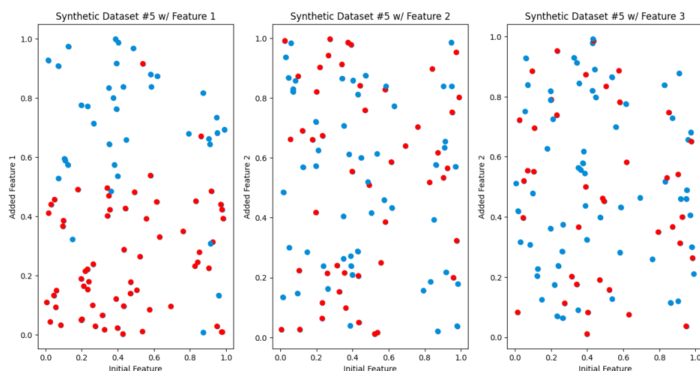
Figure 7: Synthetic dataset 5. Each scatter plot represents a different feature's predictive power. The first scatter plot demonstrates strong predictive capability, while the other two plots depict features with limited predictive utility. This visualization underscores the scenarios where one feature overpowers the other features.
