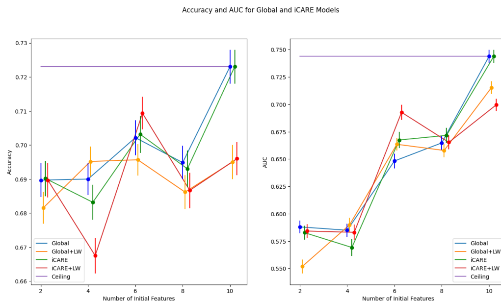
Figure 11: Heart failure dataset performance summary. This figure presents a comprehensive overview of mean accuracy and AUC metrics across various feature spaces on the heart failure dataset, offering insights into global and local perspectives depicted by blue/orange and green/red lines, respectively. Error bars show the standard deviation, while convergence towards the maximum features underscores notable trends.
