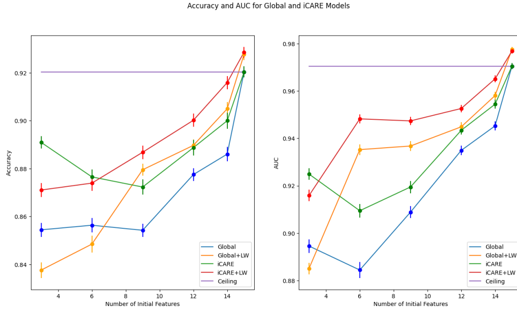
Figure 10: Early Diabetes dataset performance summary. This figure illustrates the mean performance of the early diabetes dataset on different feature spaces on accuracy and AUC metrics, with global and local perspectives represented by blue/orange and green/red lines, respectively. Error bars at each data point represent the standard deviation from the mean. The line graphs the maximum number of features towards the ceiling, represented by the purple line. The ceiling model represented an ML model trained on all features.
