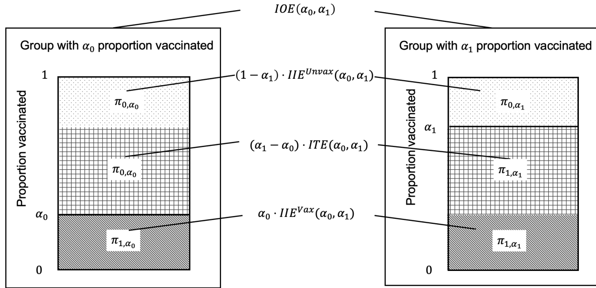
Figure 1. Graphical illustration on partitioning individual-level overall effect. Time notation ( t ) is suppressed for the ease of exposition. The two rectangles represent a pair of counterfactuals wherein the group has \alpha_0 or \alpha_1 proportion vaccinated ( \alpha_1 > \alpha_0 ). Individuals fall into three categories based on their vaccination status under the counterfactuals: 1) the dotted region represents those who are unvaccinated under both counterfactuals (hereafter referred to as “never-vaccinated”) and for whom IIE^{Unvax}(\alpha_0, \alpha_1) is in operation; 2) the gridded region represents those who are unvaccinated under \alpha_0 but vaccinated under \alpha_1 and for whom ITE(\alpha_0, \alpha_1) is in operation (hereafter referred to as “additionally-vaccinated”); and 3) the striped region represents those who are vaccinated under both counterfactuals (hereafter referred to as “always-vaccinated”) and for whom IIE^{Vax}(\alpha_0, \alpha_1) is in operation. Theorem 1 shows that IOE(\alpha_0, \alpha_1) is a weighted average of three effects: 1) IIE^{Unvax}(\alpha_0, \alpha_1) , 2) ITE(\alpha_0, \alpha_1) , and 3) IIE^{Vax}(\alpha_0, \alpha_1) , each weighted by the proportion of individuals for whom the effect is in operation respectively: 1) 1 - \alpha_1 for the never-vaccinated, 2) \alpha_1 - \alpha_0 for the additionally-vaccinated, and 3) \alpha_0 for the always-vaccinated.
