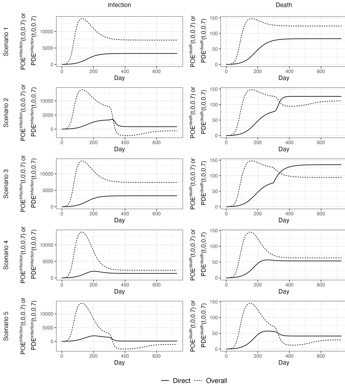
FIGURE 2. Population-level direct and overall effects given \alpha_0 = 0 and \alpha_1 = 0.7 to verify Claim 1a. Scenario 1, all parameters are time-invariant; Scenario 2, the number of effective
