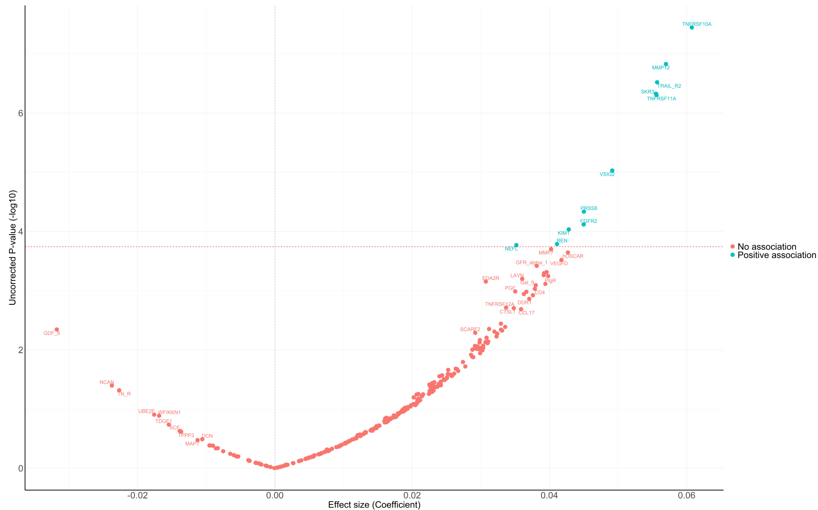
Figure 2. Volcano plot showing minimally adjusted coefficient (x axis) and uncorrected two-sided P values (y axis) for the association between protein concentration with social isolation using imputed data.
