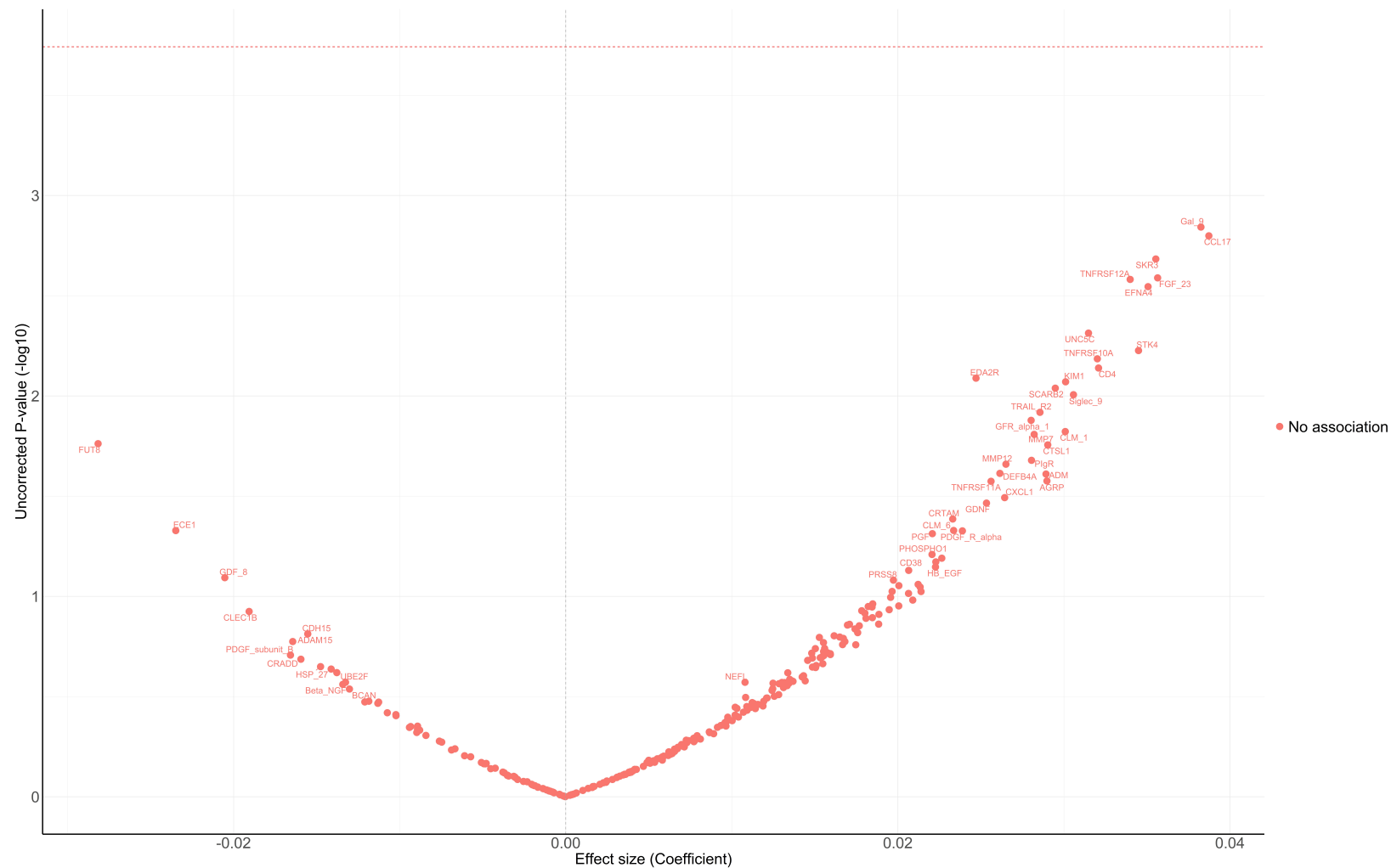
Figure 1. Volcano plot showing minimally adjusted coefficient (x axis) and uncorrected two-sided P values (y axis) for the association between protein concentration with loneliness using imputed data.
