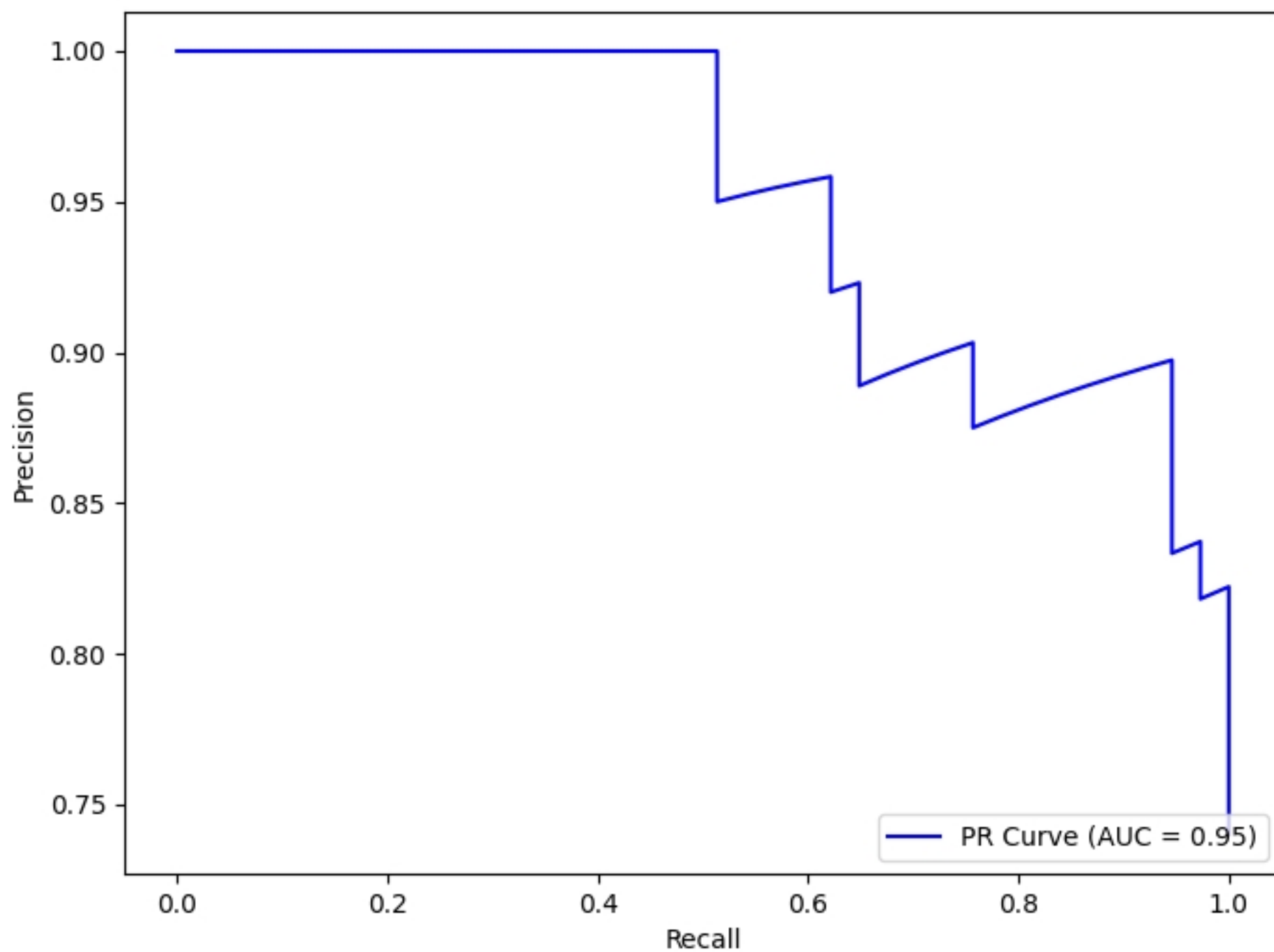
Precision-Recall Curve
