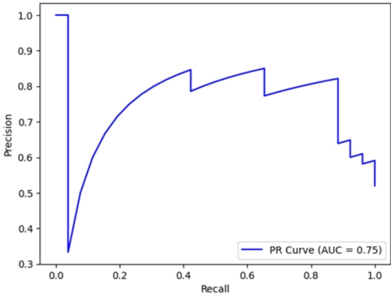
Precision-Recall Curve
