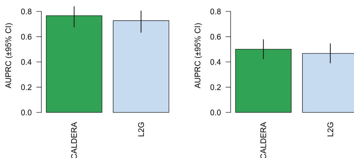
Figure 5. Area under the precision-recall curve (±95% confidence intervals) for CALDERA and L2G model predictions in A) the Open Targets ground truth dataset or B) a ground truth dataset derived from burden tests of rare coding variants in the UK Biobank.
