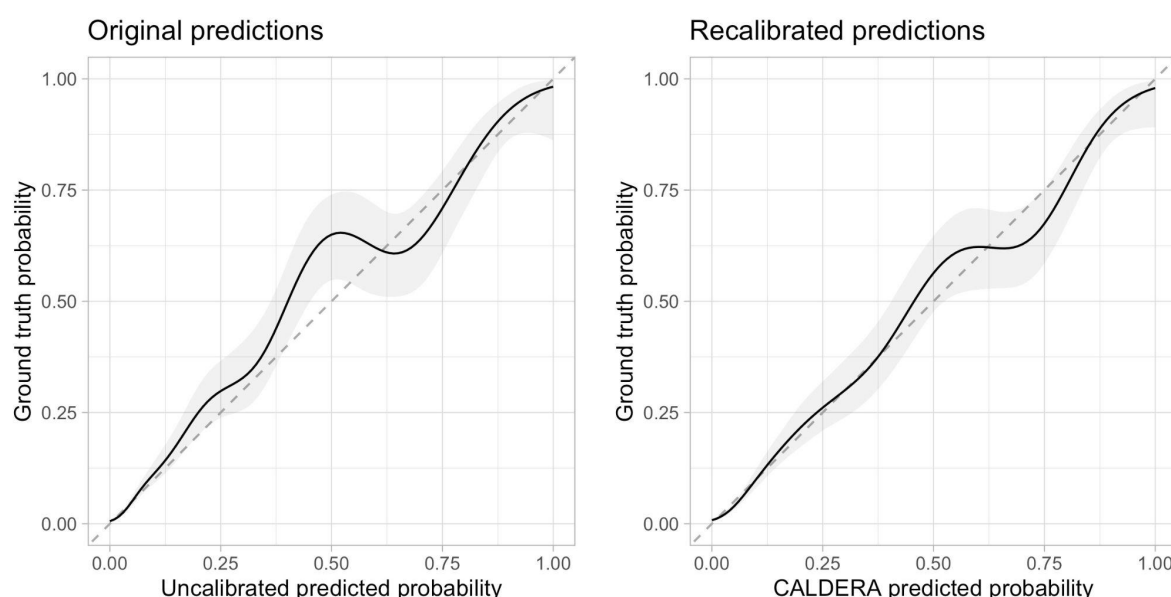
Figure 4. Calibration plots before (A) and after (B) recalibration. The x-axis represents model predicted probability in held-out trait data and the y-axis represents the ground truth causal probability. The solid lines represent the fitted value from generalized additive models with shaded areas representing 95% confidence intervals. The dashed lines represent perfect calibration.
