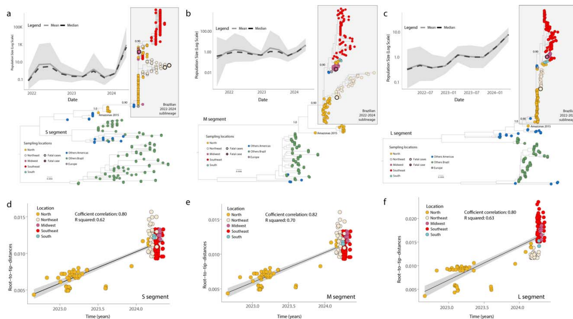
Figure 3. Molecular Evolution and Demographic History of OROV Segments S, M, and L. a1, b1 and c1) Population size of OROV infections (Log scale) over time estimated under the coalescent-based Bayesian Skygrid (BSKG) model (posterior median = solid lines, 95% HPD = pale areas) per each segments; a2, b2 and c2) Maximum likelihood phylogenetic trees of the three independent OROV segments S (n = 376), M (n = 231) (a), L (n = 303). Tips are color-coded according to the legend in the left corner; a3, b3 and c3) Regression of sequence sampling dates against root-to-tip genetic distances in a maximum likelihood phylogeny of the Brazilian 2022-2024 expansion clade (n=254).
