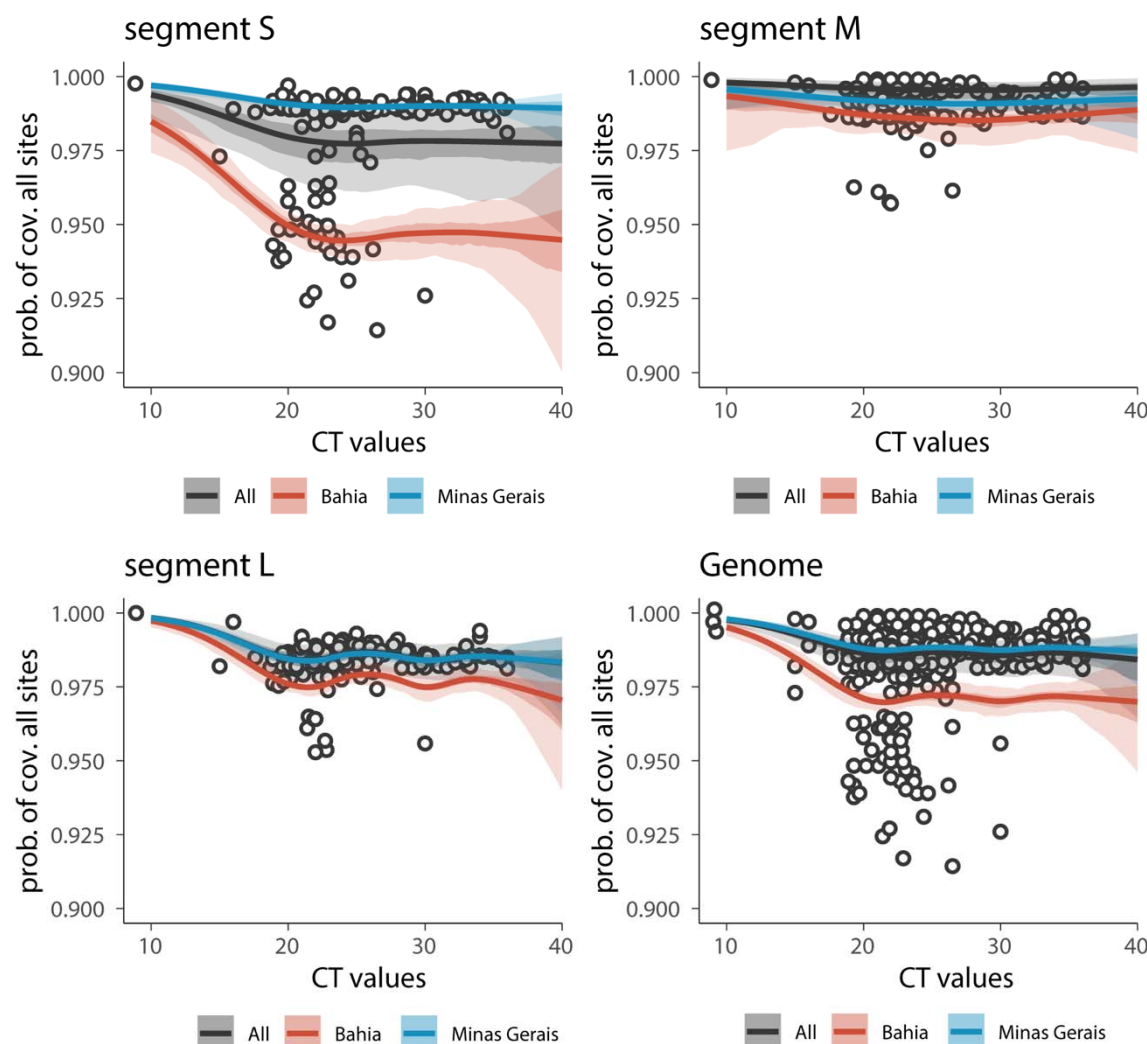
Figure S2. Sequence Coverage Probability Across Genome Segments in Different Brazilian States. The figure displays the probability of coverage for all sites across four different genome segments (S, M, L, and the entire genome) in relation to the CT value. The probability was estimated using a Generalized Additive Model (GAM; as done previously e.g. for CHIKV sequencing data [Giovannetti et al Emerg Infect Dis. 2023;29(9):1859-1863]). The GAM was defined with a binomial family, with coverage modelled as the proportion of sites recovered from sequencing, using sample state (Brazilian state) as random effect. Solutions presented (in color) include the specific ones for the two states with most sequencing (Bahia, red; Minas Gerais, blue) and the general model output (gray).
