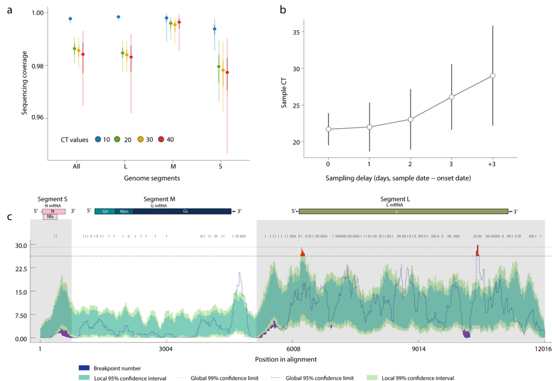
Figure 2. Sequencing coverage and recombination plot and across genome segments. a) Summary of estimated sequence coverage dependent on sample CT using a Generalized Additive Model. Shown are the mean (points) and 95% CI (ranges) for model estimates given selected values of CT (10, 20, 30, 40, in color) for all segments separately and together; b) Sample CT values (mean as points, standard deviation as ranges) plotted against the sampling delay (days between symptom onset and sample collection). c) Black lines above the figure indicate detected breakpoint positions. The green pearl aqua region shows the 95% confidence interval for expected breakpoint clustering under random recombination, while the tea green region represents the 99% confidence interval. The lower and upper dashed lines denote the 95% and 99% confidence intervals, respectively. The blue line represents the total number of breakpoints per 200-nucleotide window across the genome. Regions where the blue line exceeds the green pearl aqua area are highlighted in orange as recombination hotspots. Regions where the blue line falls below the tea green area are marked in purple as recombination cold spots.
