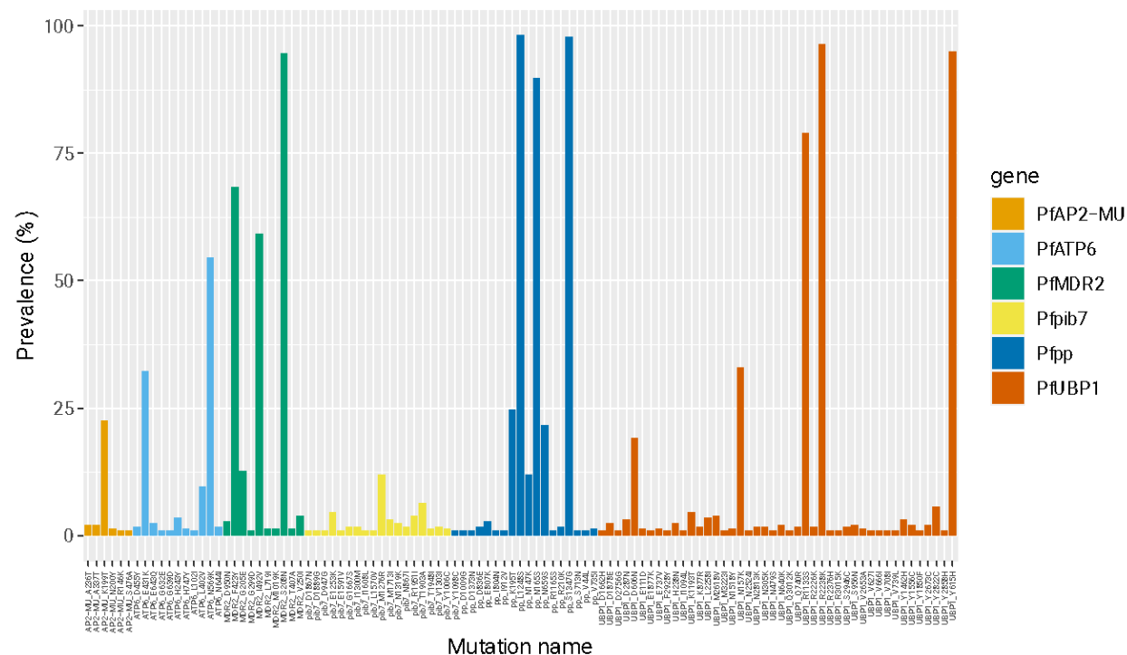
Figure S5. Prevalence of different mutations across genes associated with partial artemisinin resistance other than Kelch13 gene. We identified several mutations across PfATPase6 protein, apicoplast ribosomal protein S10 precursor gene ( Pfarps10 ), ( Pfmdr ) protein 2 codon, AP-2 complex subunit mu gene ( Pfap2-mu ), ubiquitin carboxyl-terminal hydrolase 1 gene ( Pfubp-1 ) and Phosphoinositide-binding protein ( Pfpib7 ). No mutation observed in genes: Pfcrt I356T, Pfffd D193Y, Pfmdr2 T484I, Pfap2-mu S160N/T and Pfubp-1 E1528D – known background mutations associated with ART in SEA. Also, no mutation was observed in the AP-2 complex subunit mu gene (ap2-mu, S160N/T) and the ubiquitin carboxyl-terminal hydrolase 1 gene (ubp-1, E1528D), mutation that is associated with delayed ACT clearance in Africa.
