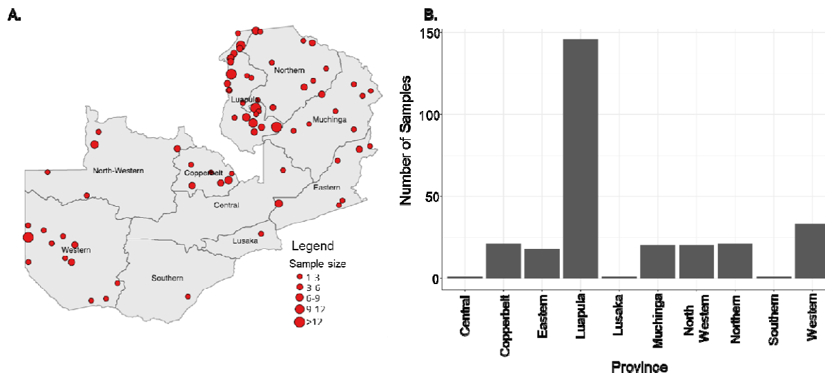
Figure 1: Spatial distribution of samples retained (n=282) for downstream drug resistance analysis. A) Sample distribution at the cluster level across Zambia. The size of each sample collection cluster (red) is shown in proportion to the cluster sample size. B) Sample size per
