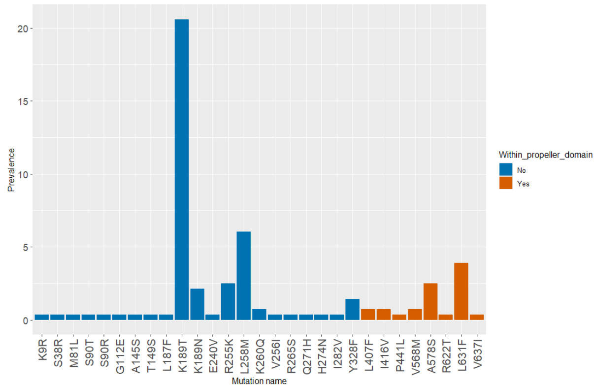
Figure 4. Non-synonymous mutations identified across the kelch13 gene in Zambia. Colors indicate mutations as outside (blue) or within (orange) the propeller domain.
