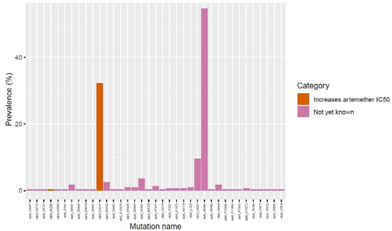
Figure S4. Prevalence of 37 mutations in Pfatpase6 from 282 Zambian samples ordered by genomic loci. Colours indicate whether the mutations are validated or not as resistance markers for ACT.
