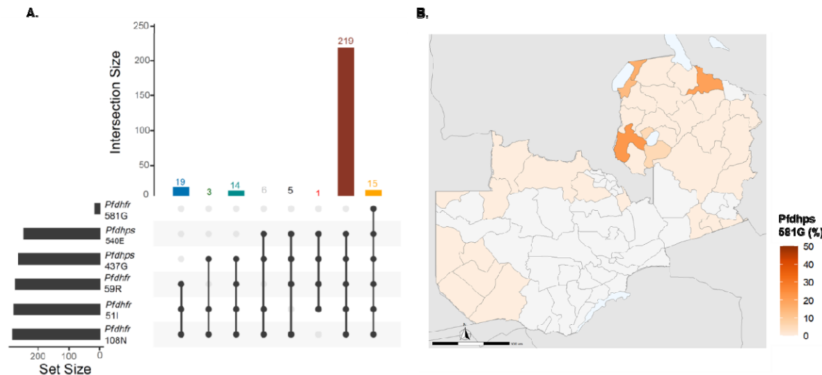
Figure 3. Cumulative prevalence of Pfdhfr - dhps mutations (A) and spatial prevalence of Pfdhps A581G (B) across Zambia. Color code heat map shows prevalence at the district-level, while white indicates districts where no samples were available.
