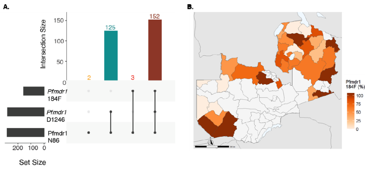
Figure 5. Prevalence of Pfmdr1 mutations associated with decreased sensitivity to lumefantrine. A) Cumulative prevalence of Pfmdr1 haplotypes, B) Spatial prevalence of the Pfmdr1 184F mutation. Color code heat map shows the prevalence at the district level, while white indicates districts where no samples were available.
