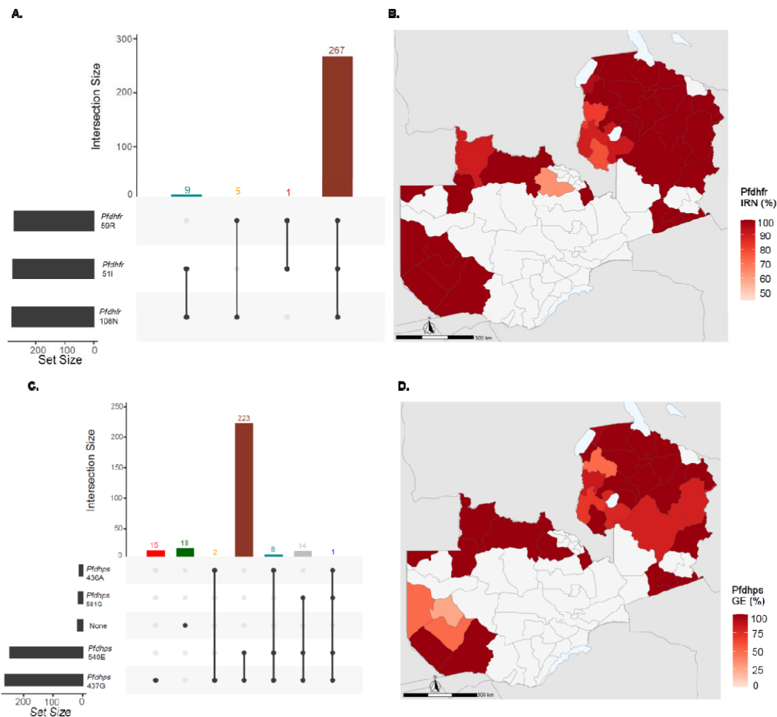
Figure 2. Prevalence of Pfdhfr and Pfdhps mutations across Zambia. UpSet plots showing the number of times each combination of mutations was seen for Pfdhfr (A) and Pfdhps (C). The lines and circles below the bars represent the different combinations of resistant genotype in individual samples. B) Spatial prevalence of pyrimethamine resistant triple mutant ( Pfdhfr 51I/59R/108N, IRN), D) Spatial prevalence of sulfadoxine resistant double mutant ( Pfdhps 437G/540E, GE). Color code heat map shows prevalence at the district level, while white indicates districts where no samples were available.
