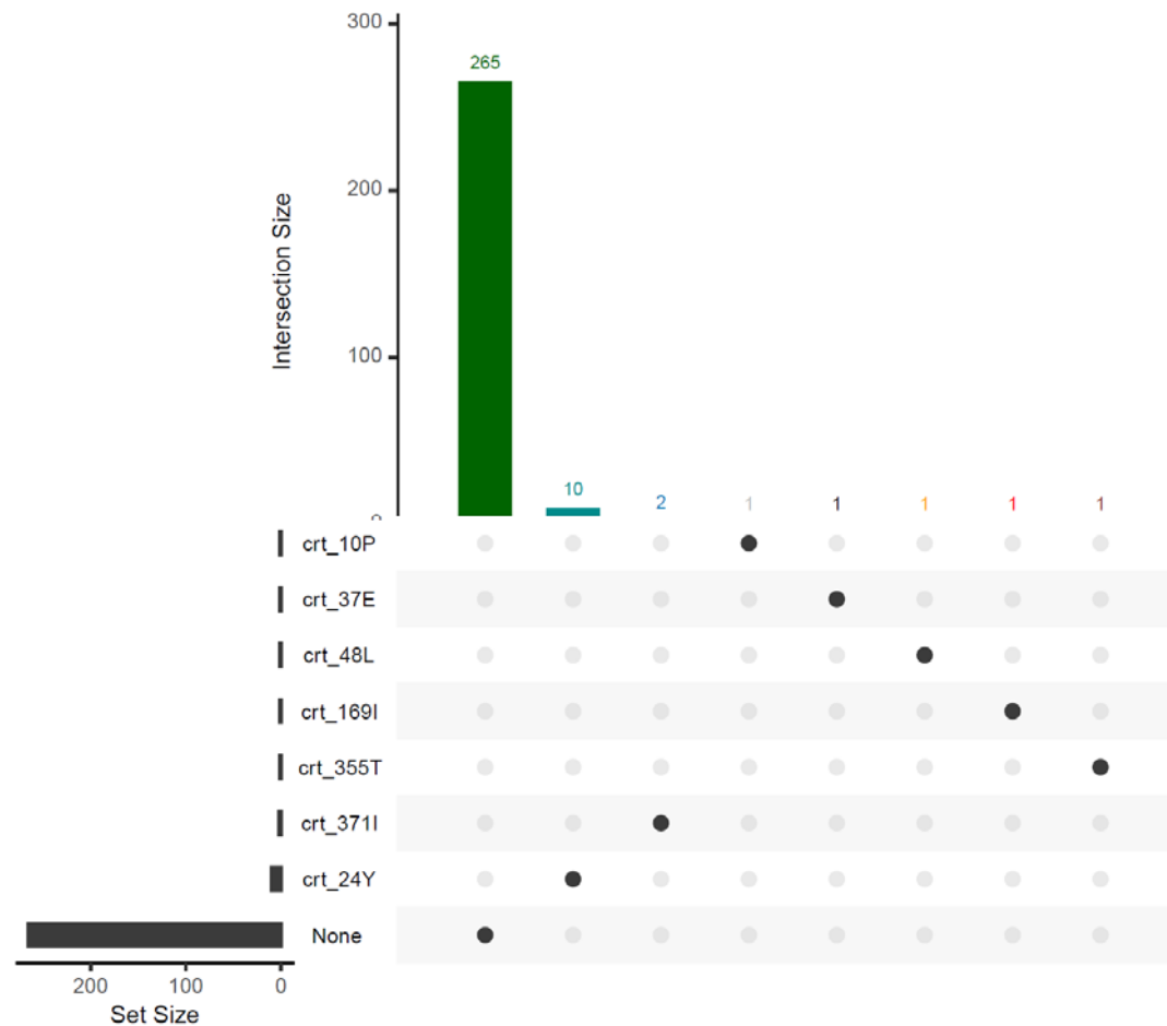
Figure S3. Frequency of mutations in the PfCRT gene. The intersection size bar plots represent the number of parasites carrying different combinations of antimalarial drug resistance associated mutations in the PfCRT gene. The circles below the bars represent the different combinations of resistant genotypes in individual samples. The set size represents the number of samples in which individual drug resistance-conferring markers were genotyped. Gene position and nucleotide change for each mutation are shown in Table S1. None = samples carrying synonymous mutations or wild-type alleles
