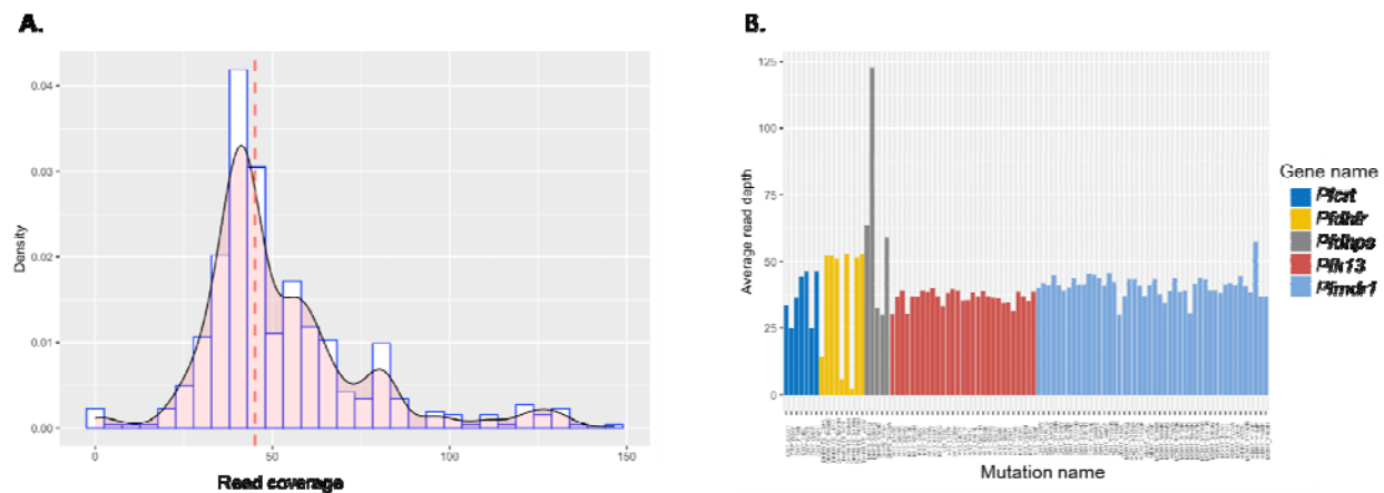
Figure S1. Read coverage per all identified mutations associated with antimalarial drug resistance across 282 samples. A) Density plot showing cumulative read depth and dashed red lines indicate median coverage=45X. B) Read coverage per mutation for top 5 known antimalarial drug resistance genes.
