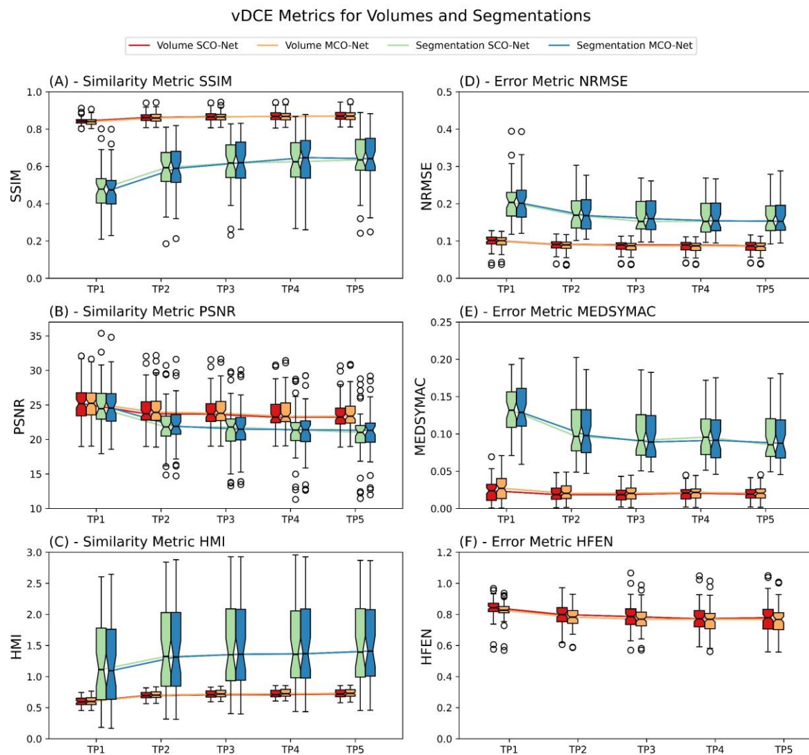
Fig. 3. Similarity metrics for vDCE SCO-Net and MCO-Net in image volume as well as segmented findings are presented. SSIM values show an increase and PSNR values a decrease for later time points both for the volume and segmentations.
