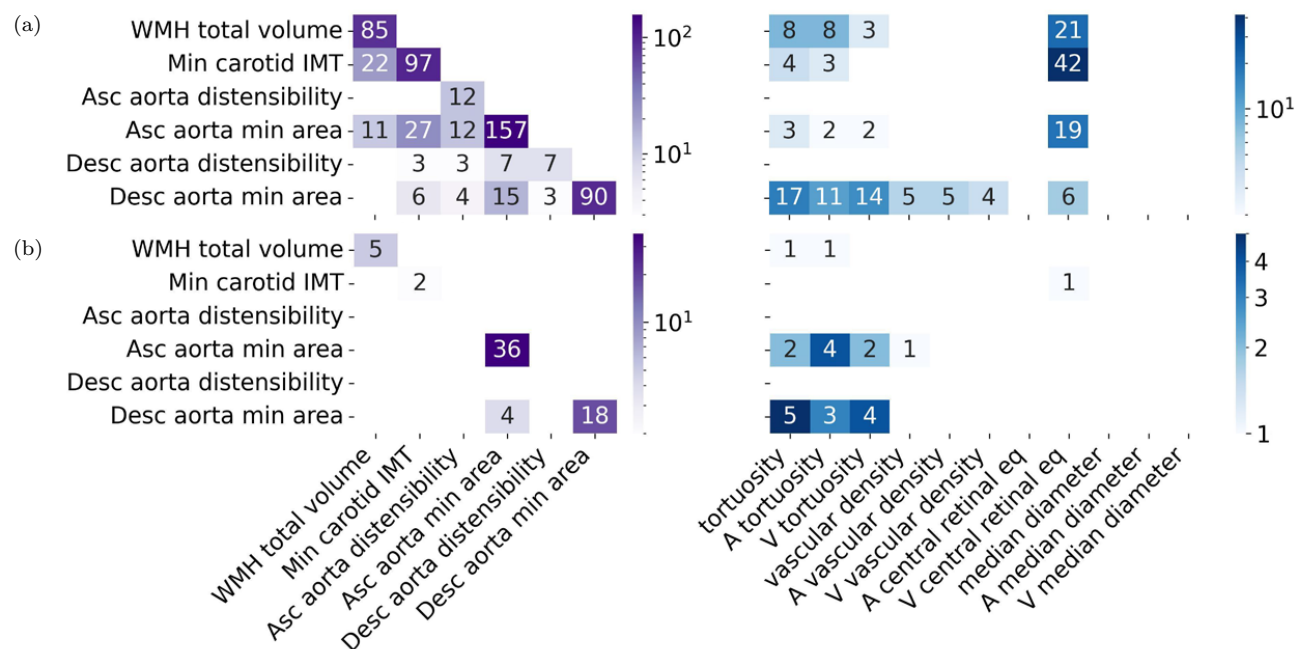
Figure 3: a) Gene-scoring intersection showing genes in common between non-retinal IDPs and non-retinal IDPs ( left ), and between non-retinal IDPs and retinal-IDPs ( right ). The diagonal ( left ) shows the number of genes significantly associated with each IDP. While the other cells show the number of intersected genes in IDP pairs. b) Pathway-scoring intersection showing pathways in common between non-retinal IDPs and non-retinal IDPs ( left ), and between non-retinal IDPs and retinal-IDPs ( right ). The diagonal ( left ) shows the number of pathways significantly associated with each IDP. While the other cells show the number of pathways in the intersection between pairs of IDPs. Genes and pathways results were obtained using PascalX [33].
