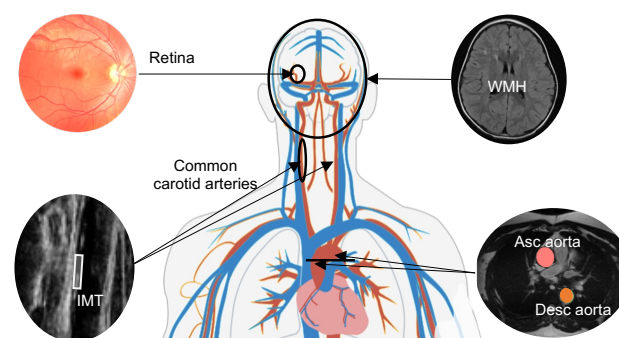
Figure 1: Visualization of the human vascular system and the imaging modalities available in the UKBB. The modalities include CFIs for examining the retina’s vasculature, ultrasound for assessing the common carotid arteries (in particular, the IMT), transverse cardiac MRI for evaluating the aorta, and structural brain MRI for detecting WMH.
