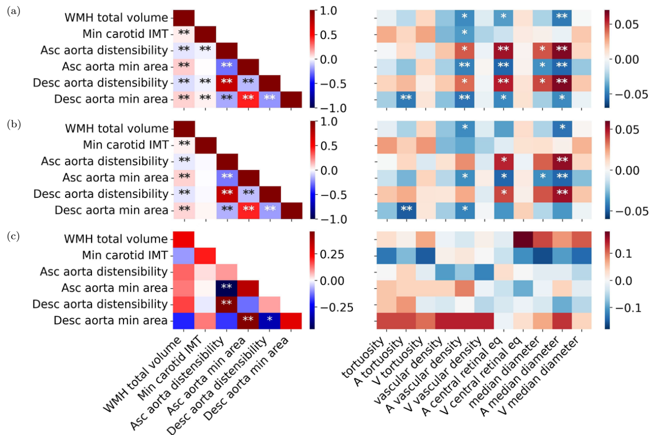
Figure 2: a) Phenotypic correlation of non-retinal IDPs with non-retinal IDPs ( left ) and retinal IDPs ( right ). b) Phenotypic correlation of non-retinal IDPs with non-retinal IDPs ( left ) and retinal IDPs ( right ) adjusted for hypertension in addition to the previous covariates. Hypertension was defined as having a systolic blood pressure (SBP) \geq 140 mmHg or diastolic blood pressure (DBP) \geq 90 mmHg. c) Genetic correlation of non-retinal IDPs with non-retinal IDPs ( left ) and retinal IDPs ( right ), computed using LDSR [30]. The diagonal of the left figure shows the heritability values of the non-retinal IDPs (values can be found in Supplementary Data ‘Heritabilities’). GWAS summary statistics from previous studies were used to conduct this analysis (see section 4), for the brain IDPs, the GWAS sample size used was around \sim 33,000 participants, for IMT around \sim 44,000 , for aortic IDPs \in (33,000-38,000) , and retinal IDPs \in (54,000-69,000) . For all the images, the x-axis shows non-retinal IDPs ( left ) and retinal IDPs ( right ) and the y-axis shows non-retinal IDPs. Colors indicate standardized effect sizes for linear regressions (a, b) or the genetic correlation coefficient (c), while asterisks indicate the level of statistical significance (except for the diagonal of figure c). These p-values were corrected for multiple testing ( * : p < 0.05/N_{test} , ** : p < 0.001/N_{test} , where N_{test} (= 84) = N_{IDPs} \times (N_{IDPs}/2 + N_{retina}) ). All IDPs were adjusted for covariates (see section 4). For more details, see Supplementary Data ‘Main IDPs information’.
