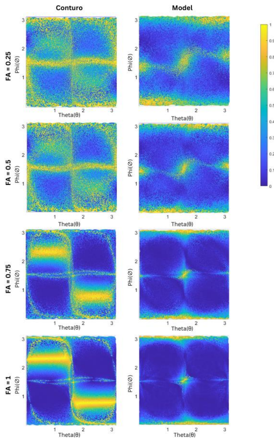
Figure 5. Angular error as the cosine distance between the predicted principal eigenvector and the true vector for various orientations of the vector (\theta, \Phi) . Trace = 0.0021 mm 2 /s. One of the gradient axes was rotated 12 degrees in the x-axis to simulate transform
