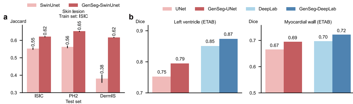
Extended Data Fig. 1 | a. Comparison between GenSeg-SwinUnet and SwinUnet models, both trained on 40 examples from the ISIC dataset and evaluated on the test sets of ISIC, PH2, and DermIS. b. The performance of GenSeg applied to UNet (GenSeg-UNet) and DeepLab (GenSeg-DeepLab) under in-domain settings (test and training data are from the same domain) in the tasks of segmenting left ventricles and myocardial wall using 8 training examples from the ETAB dataset, compared to vanilla UNet and DeepLab.
