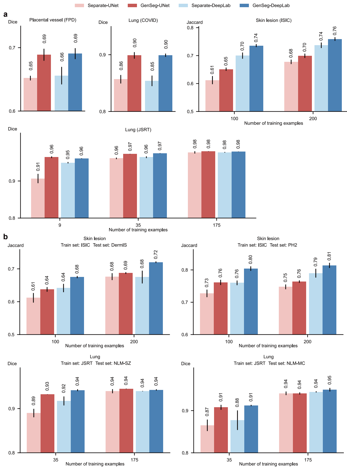
Extended Data Fig. 7 | Further comparison of GenSeg's end-to-end data generation mechanism with baselines' separate generation mechanism. a, GenSeg's end-to-end generation mechanism greatly improves models' in-domain generalization performance, when used UNet and DeepLab in segmenting placental vessels, lung regions, and skin lesions using FPD, COVID, ISIC, and JSRT datasets. b, GenSeg's end-to-end generation mechanism greatly improves models' out-of-domain generalization performance, when used UNet and DeepLab in segmenting skin lesions (using ISIC for training, and DermIS and PH2 for testing), and lung regions (using JSRT for training, and NLM-SZ and NLM-MC for testing).
