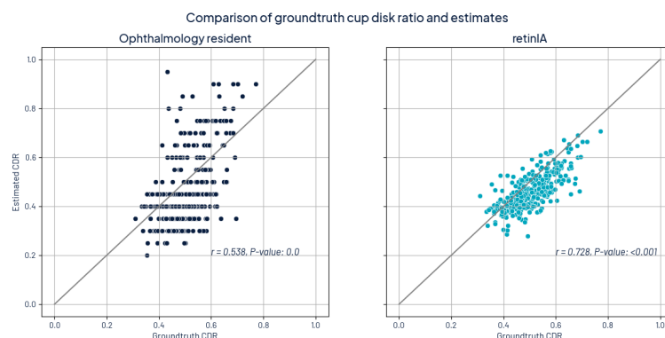
Figure 2: Comparison of CDR estimates with groundtruth CDR. The left image shows the comparison with the residents of ophthalmology and the right image shows the comparison with retinIA.
