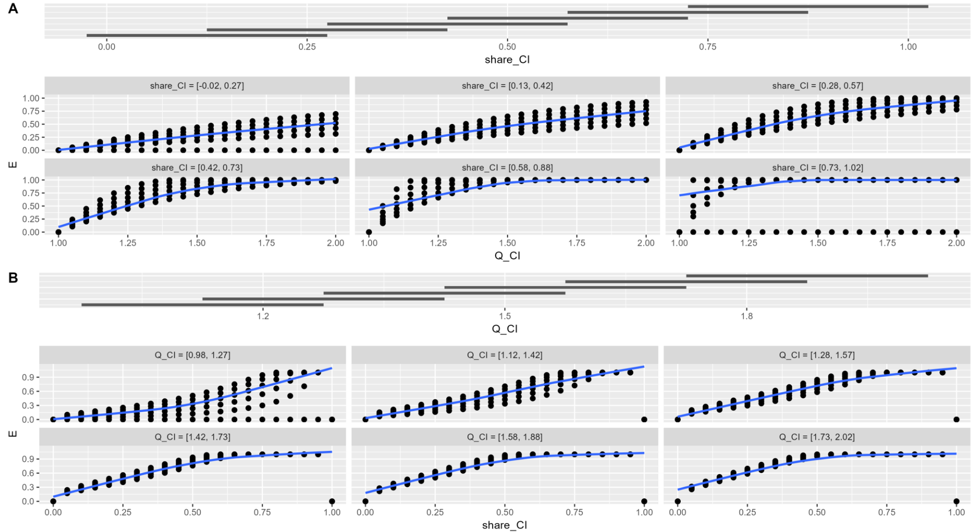
Figure 2 (A) Coplot of efficacy (E) versus the relative nutrient intake increase (Q_CI) controlling for the relative nutrient intake gap (CI%). (B) Coplot of efficacy (E) versus the relative nutrient intake gap (CI%) controlling for the relative nutrient intake increase (Q_CI).
