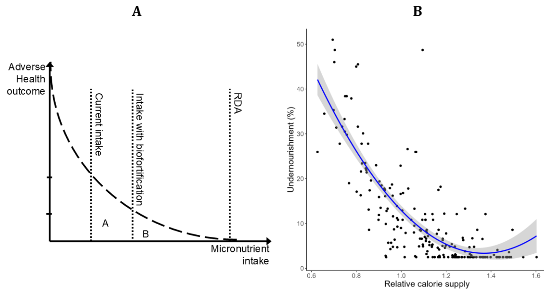
Figure 1 (A) Conceptual relationship between adverse health outcome and relative nutrient intake (source: Stein et al. (2005)). (B) Empirical relationship between the prevalence of undernourishment and relative calorie intake (source: own calculation following Fischer et al. (2005)).
